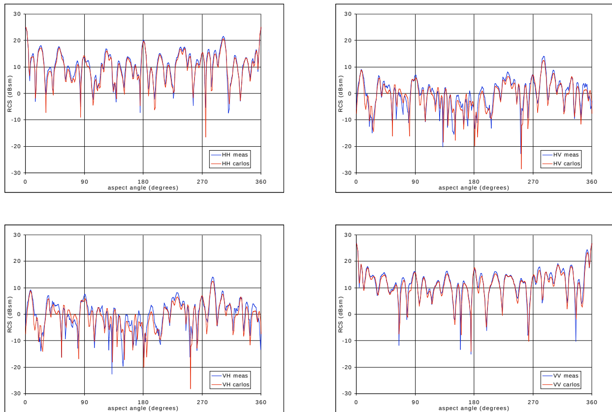
Figure 5: Polarimetric RCS of Slicy at 286 MHz. (The data have been adjusted to represent VHF/UHF data by assuming the model in Fig. 4 was a 1/35 th scale Slicy, i.e. 10\log(35^2) was added to the measured RCS).
