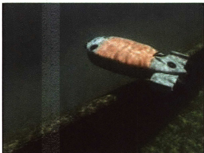
FIGURE 1-2: CETUS II VEHICLE
