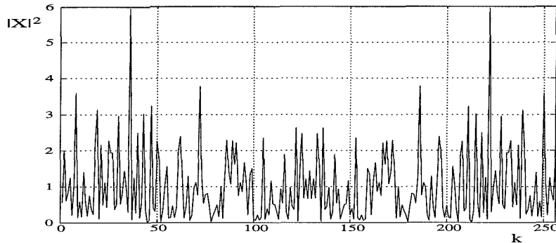
Figure 2: Periodogram of a pseudorandom sequence
