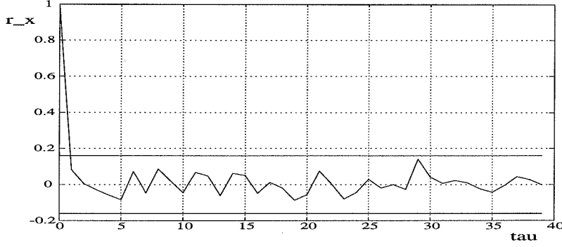
Figure 1: Autocorrelation plot of a pseudorandom sequence
