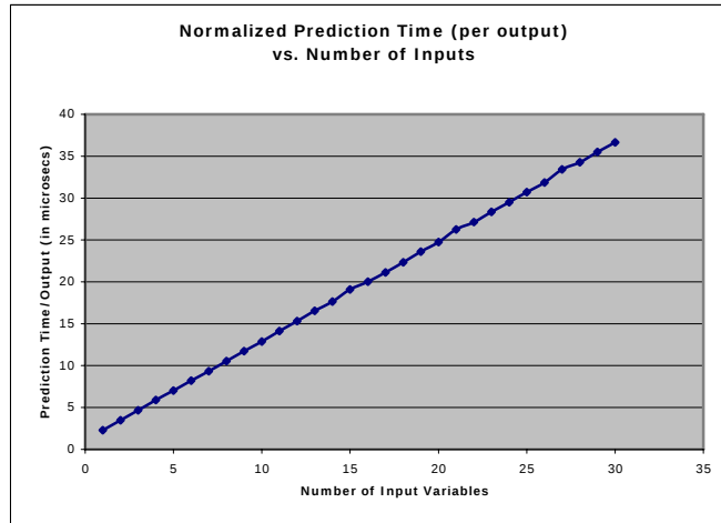
Figure 14. Prediction time for each output variable increases linearly with input parameters.
