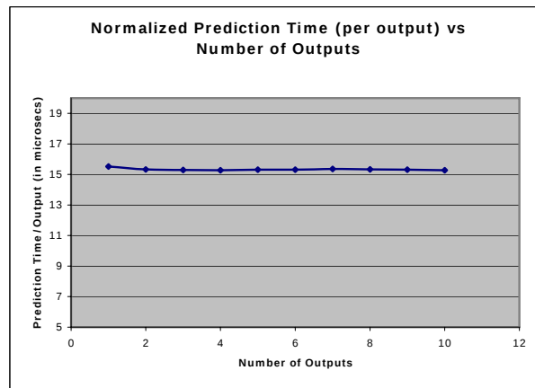
Figure 15. Prediction time for output variables is independent of the number of output variables.
