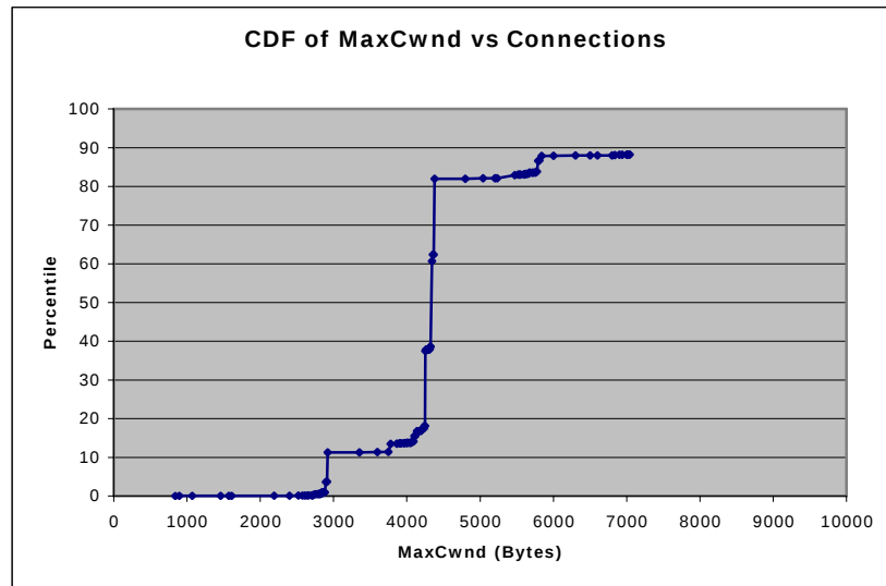
Figure 5. Most connections have a small congestion window. Only connections with large enough window can benefit from tuning.
