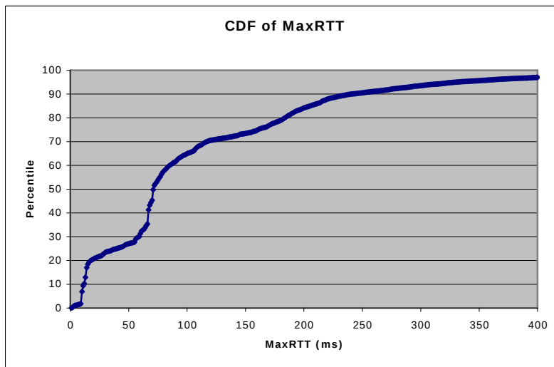
Figure 7. ALN can improve connections that last long enough to open the congestion window but short enough that transients dominate.
