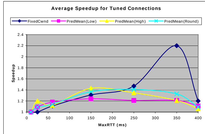
Figure 20. Speedups observed are best for RTTs in the middle of the RTT range. The speedups range from 1.1x to 2.2x with an average around 1.2x.
