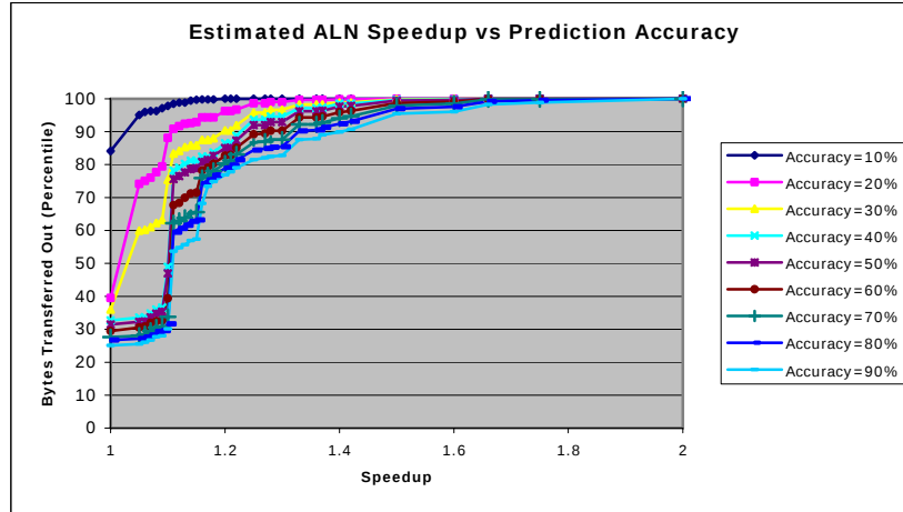
Figure 13. Poor (under)prediction is better than none. Fair prediction can add another 20% improvement.
