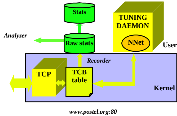
Figure 1. Experimental setup that combines Web100 kernel instrumentation with ALN in the user space.
