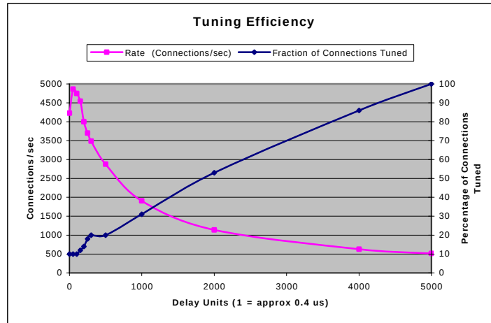
Figure 18. At high rates, most connections to untuned because of high load.
