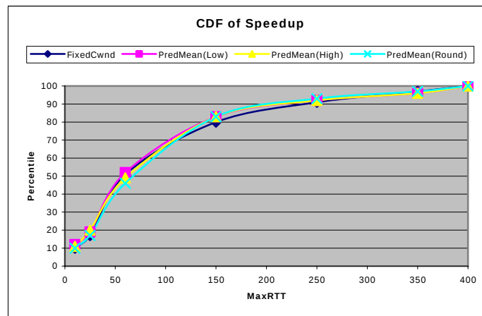
Figure 20. Speedups observed are best for RTTs in the middle of the RTT range. The speedups range from 1.1x to 2.2x with an average around 1.2x.
