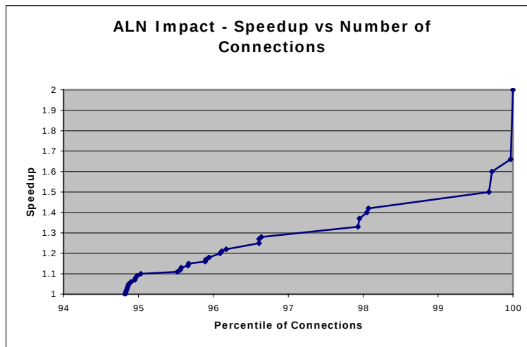
Figure 10. Potential for low load on the prediction mechanism given which of the 3-5% of connections to optimize.
