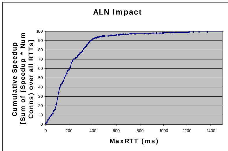
Figure 11. 70% of the bytes transferred see 20% or more gain.
