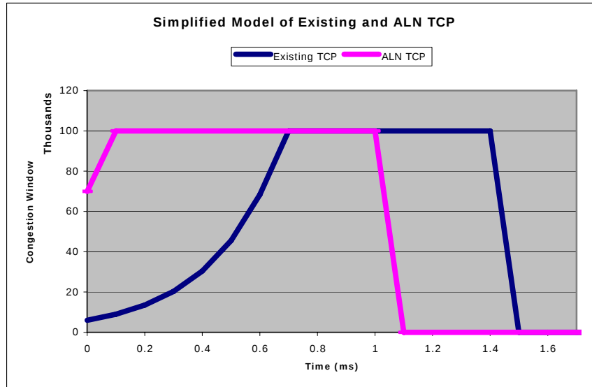
Figure 9. Simple model used to estimate potential speedup
