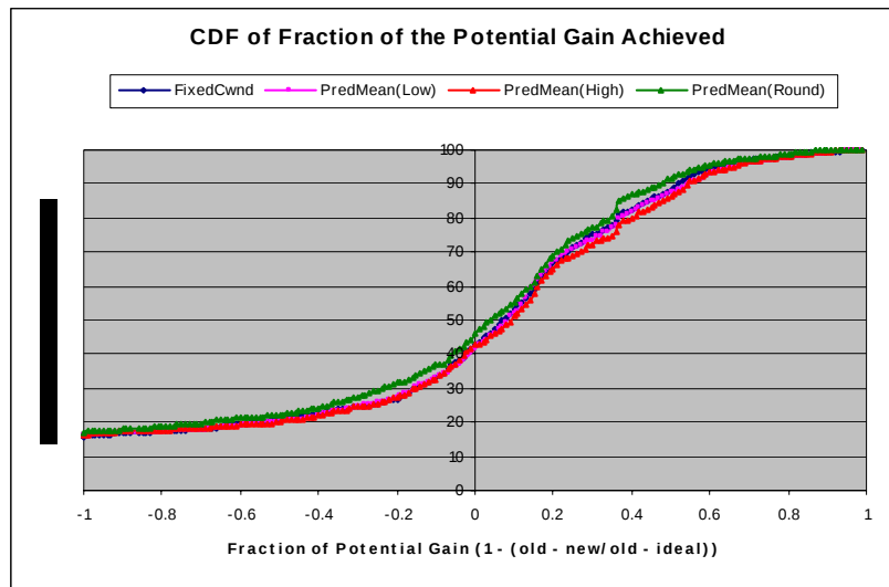
Figure 23. More work is required to accurately identify connections and conditions in which ALN can improve the performance.
