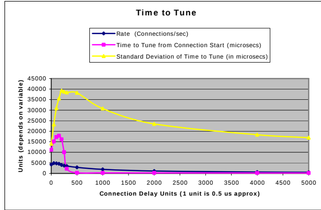
Figure 17. At high rates, the time to tune is high both in absolute terms and in terms of standard deviation. At rates \leq 500 connections/sec, the time to tune is a low fixed value (170us).
