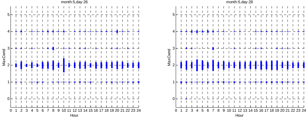
Figure 4. Data Pattern for MaxCwnd
