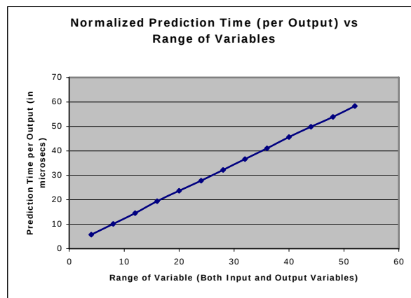
Figure 16. Prediction time for each output increases linearly with range of each variable.
