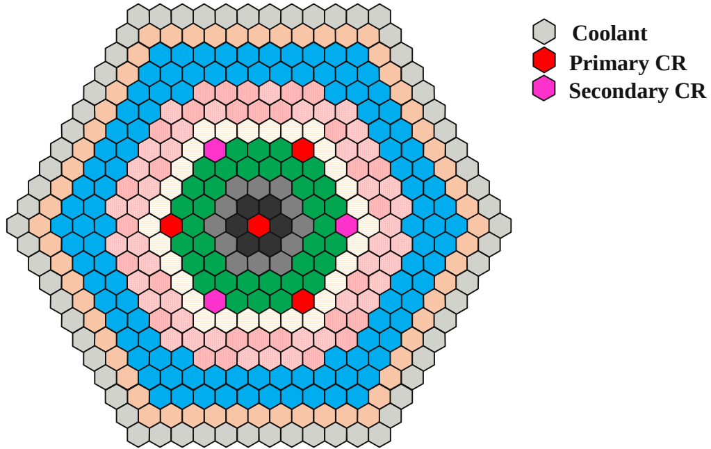
Figure 4.1 SSTAR Core Design 76
