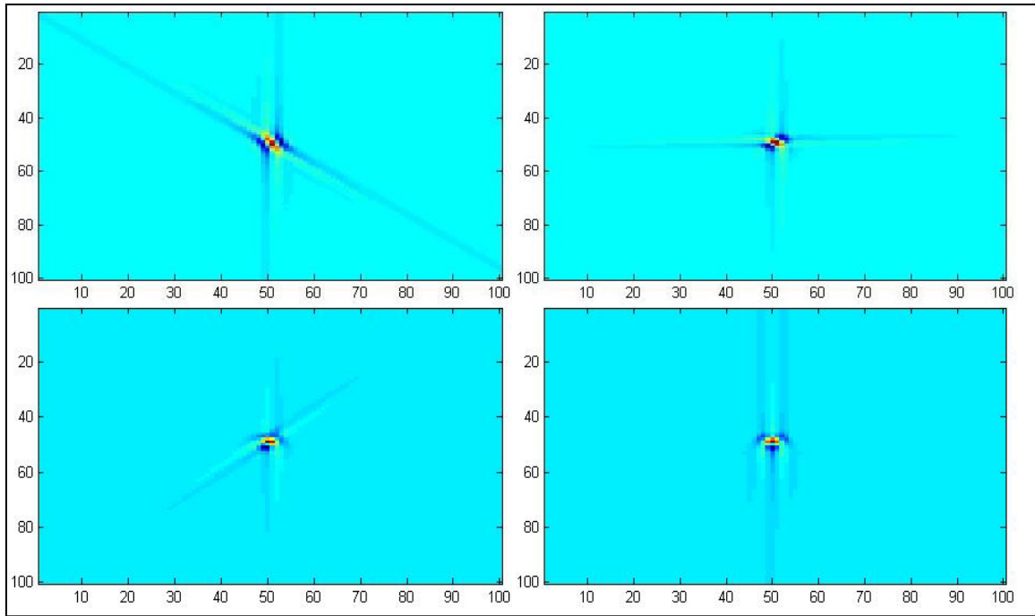
Figure 30 Image reconstruction based on 45°, 90°, 135° and 180° (starting clockwise from top-left picture) views of the target
