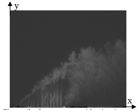
Figure 4b: Instantaneous side-view image (Case 1, P_{inj} = 144 psia)
