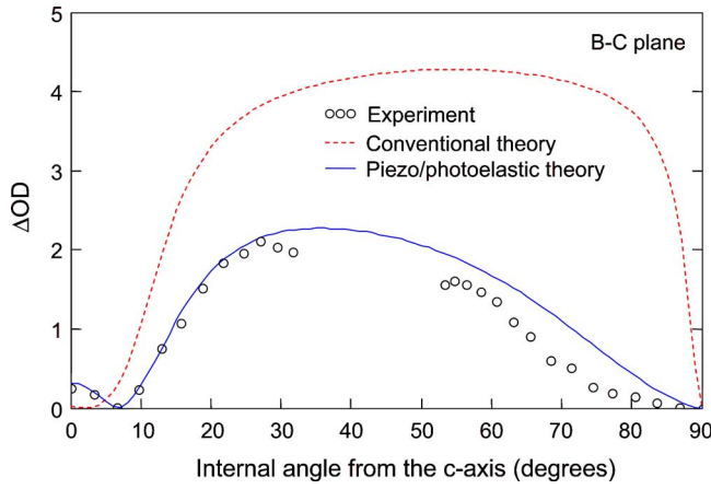
FIG. 5. (Color online) Conventional and piezoelectric/photoelastic theories compared with b - c plane data.
