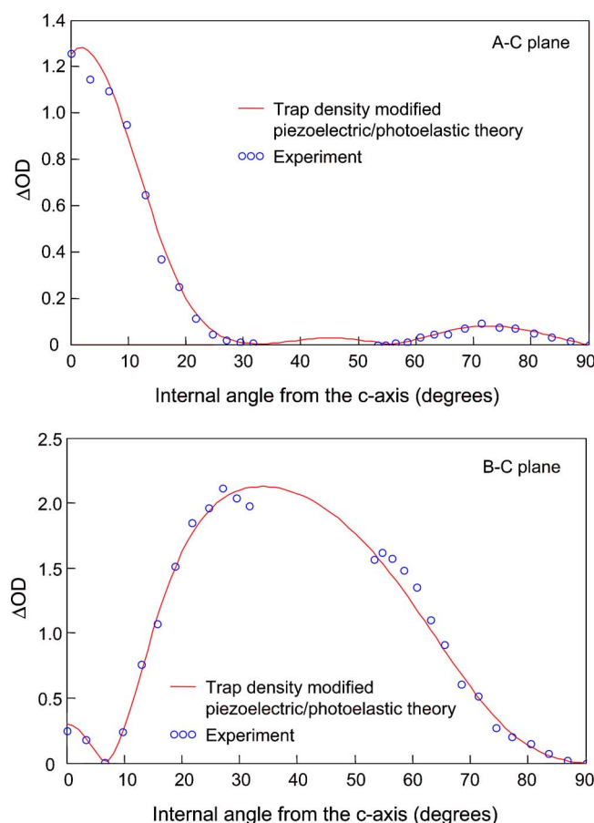
FIG. 7. (Color online) \Delta OD variation with crystal angle using the angular effective trap density measurements for the a - c and b - c crystal planes.
