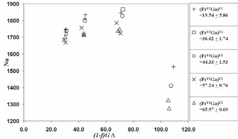
Figure 12. Nusselt number versus (1-f)G\Delta for varying (Fr^{1/2}Ga)^{1/2} .
