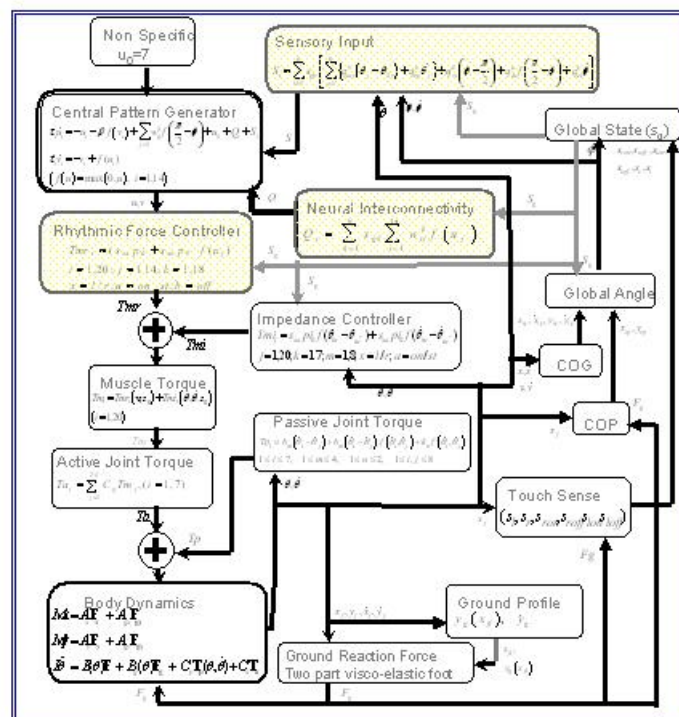
Figure 1. The basic structure of the model used in the current work. Adapted from Taga, G: Biological Cybernetics 73:97-111, 1995.
