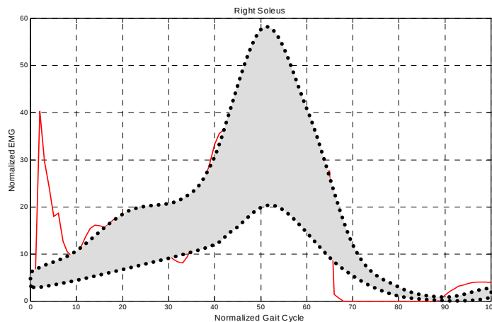
Figure 5. Representative comparison of model muscle activation to published normative data.
