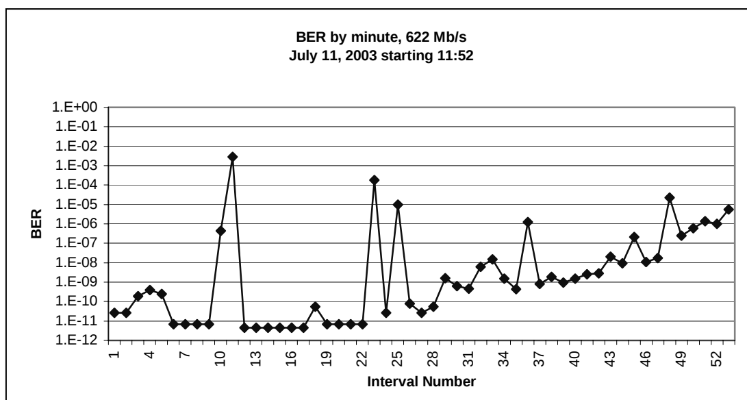
Figure 6. This graph shows how the bit error rate worsens over time for a laser data link where the beam was propagated over 16.2 km of water at the NRL Chesapeake Bay Detachment Laser Communications Test Facility (Ref. 14).
