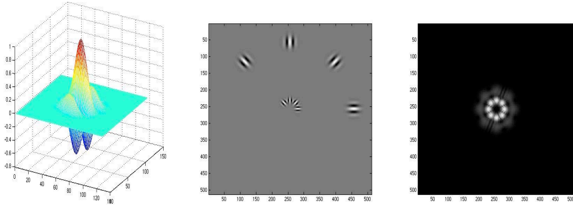
Figure 2: (a) 3-D representation of a single Gabor kernel in the spatial domain (b) 2-D spatial domain representation of a filter bank of Gabor kernels with 4 kernels placed at every 45^\circ from -45^\circ to +90^\circ at a radius of 25 and 200 pixels from the center of the image. The frequency for the inner radius is 0.8727 cycles/ degree and that of the outer radius is 0.4363 cycles/ degree (c) Frequency domain representation of (b)
