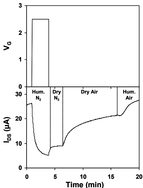
Figure 6-1. Time-dependent performance characteristics (at V_{DS} = 0.1 V) under different test conditions of a TFT device with PEDOT:PSS as the active layer and 20 PAH/PAA bilayers as the gate dielectric (deposited at a pH of 6 – 6.5 with a total thickness \sim 60 Å).
