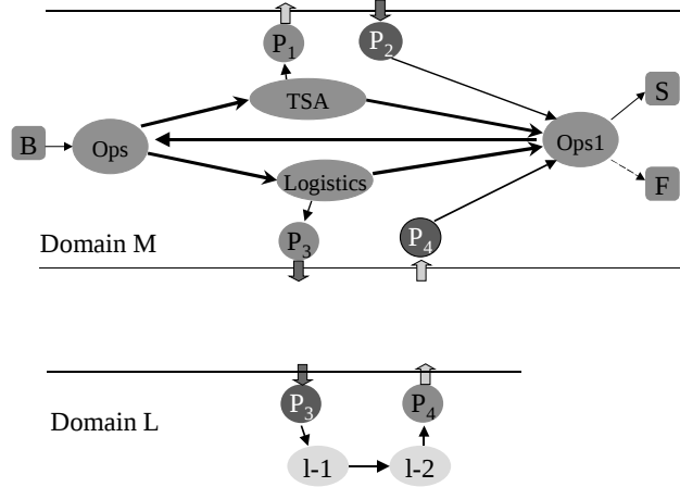
Fig. 5. An outcome of code generation from a workflow design specification
