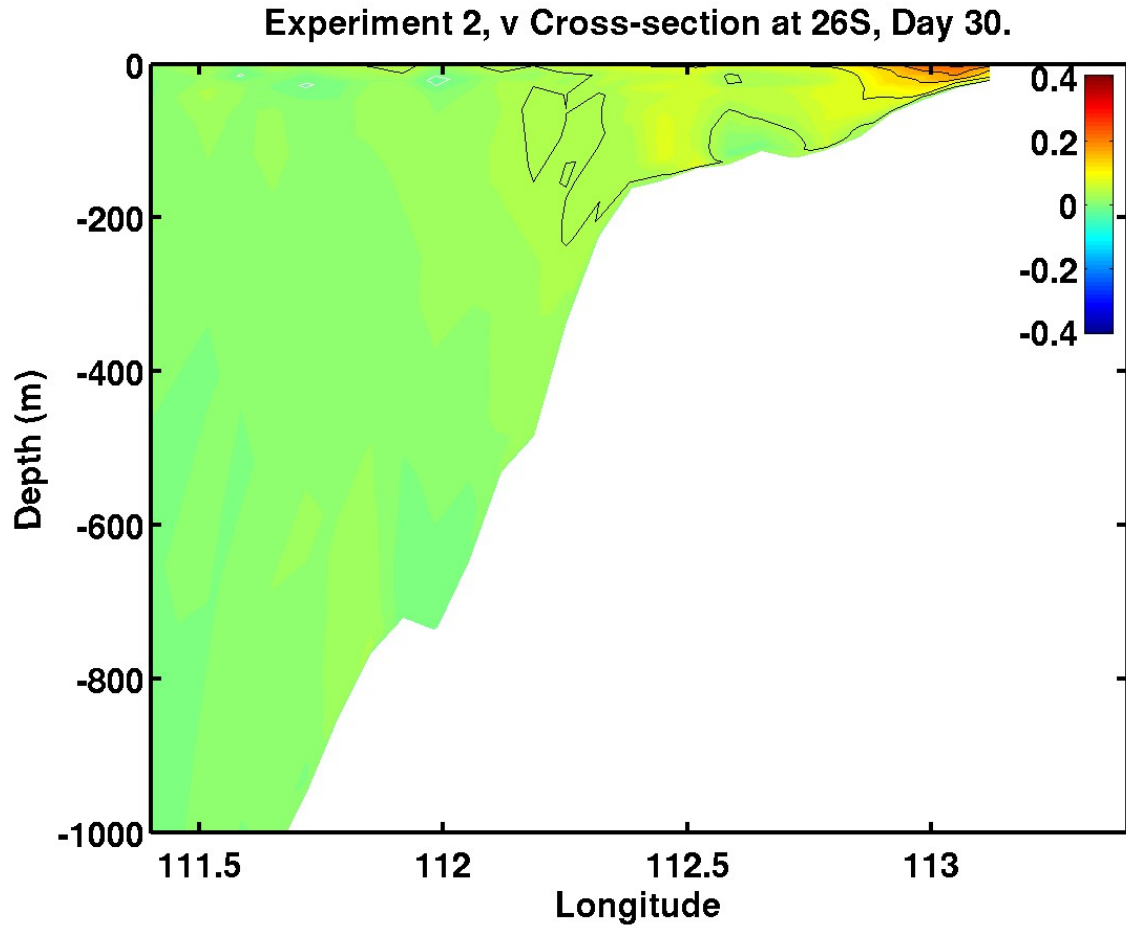
Figure 5b. Cross-section of meridional velocity component ( \text{m s}^{-1} ) at 26^{\circ}\text{S} for Experiment 2 on day 30. Red is equatorward (north) and blue is poleward (south). The white contour is zero.
