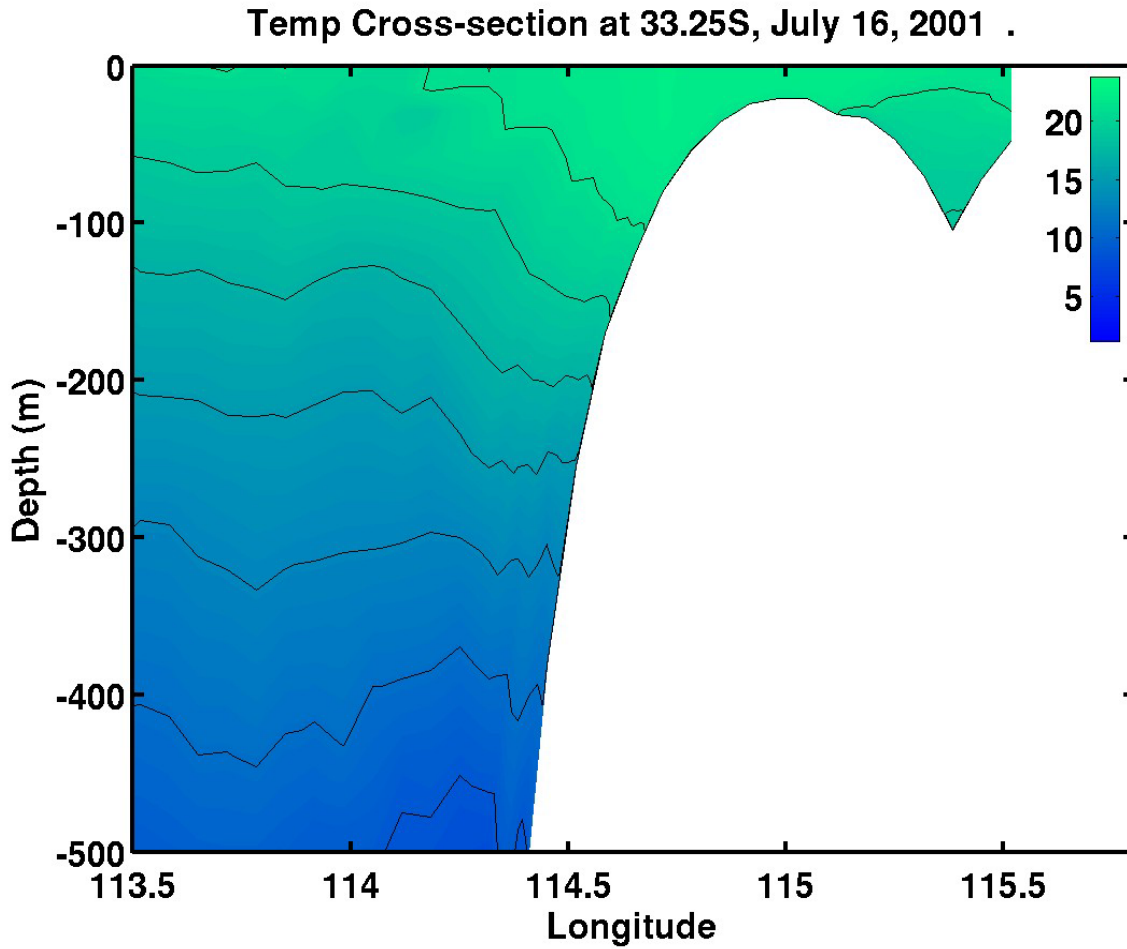
Figure 5.19d. Cross-section of temperature ( ^{\circ}\text{C} ) along an east-west transect just north of Cape Leeuwin at 33.25^{\circ}\text{S} for daily wind Experiment 4 on day 45, July 16, 2001.
