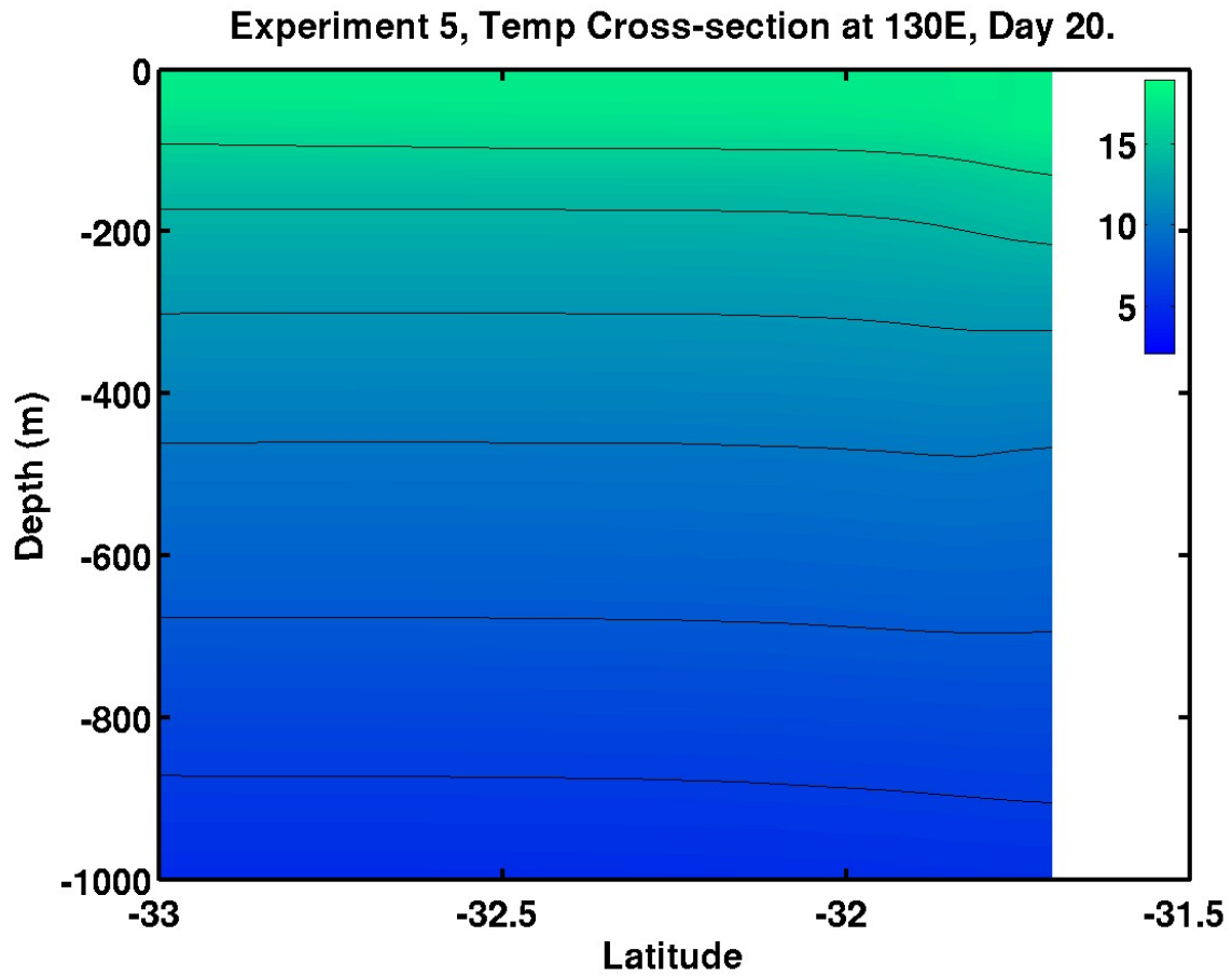
Figure 4.15g. Cross-section of temperature ( ^{\circ}\text{C} ) along an north-south transect in the Great Australian Bight ( 130^{\circ}\text{E} ) for Experiment 5 on day 20.
