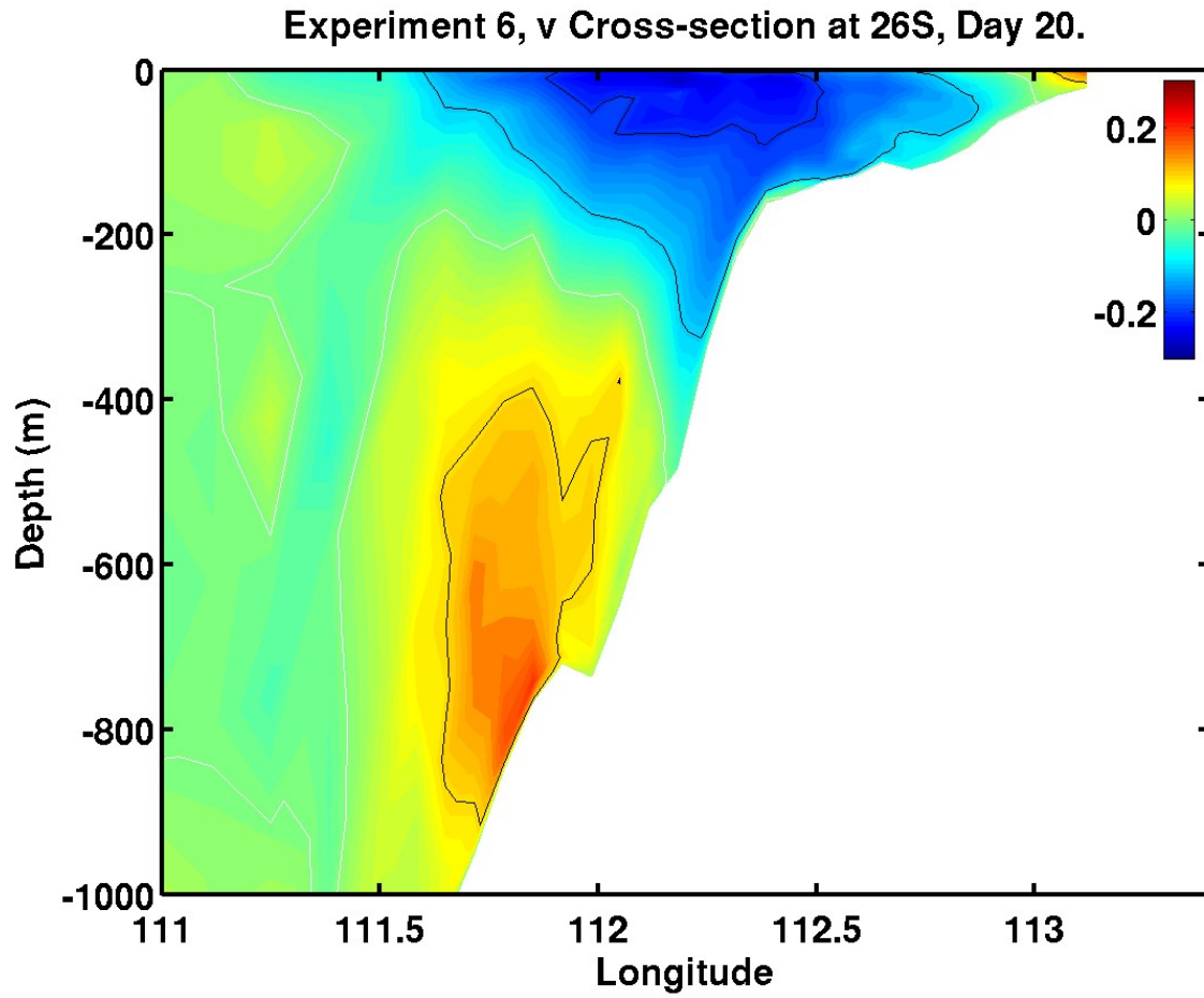
Figure 4.20b. Cross-section of meridional velocity component ( \text{m s}^{-1} ) at 26^{\circ}\text{S} for Experiment 6 on day 20. Red is equatorward (north) and blue is poleward (south). The white contour is zero.
