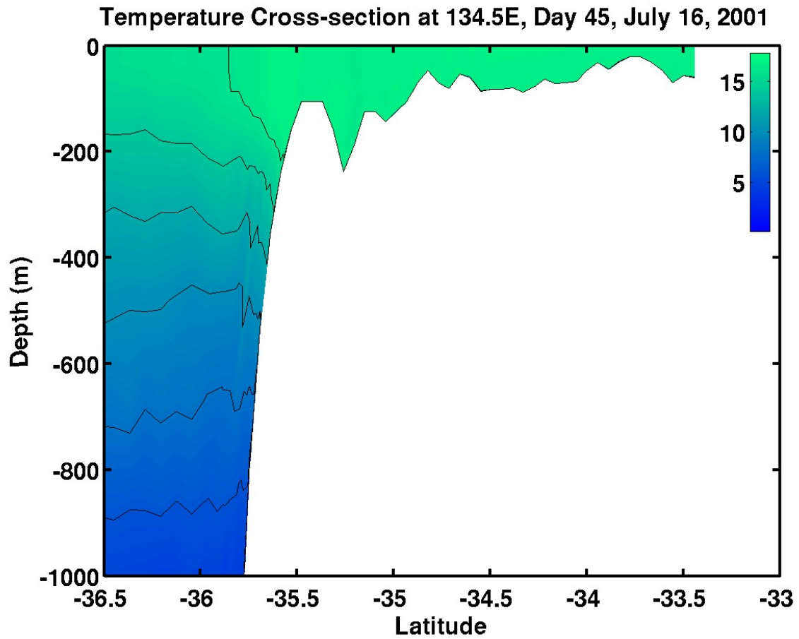
Figure 6.3a. Cross-section of temperature ( ^{\circ}\text{C} ) in the eastern Great Australian Bight ( 134.5^{\circ}\text{E} ) for daily wind Experiment 4 on day 45, July 16, 2001.
