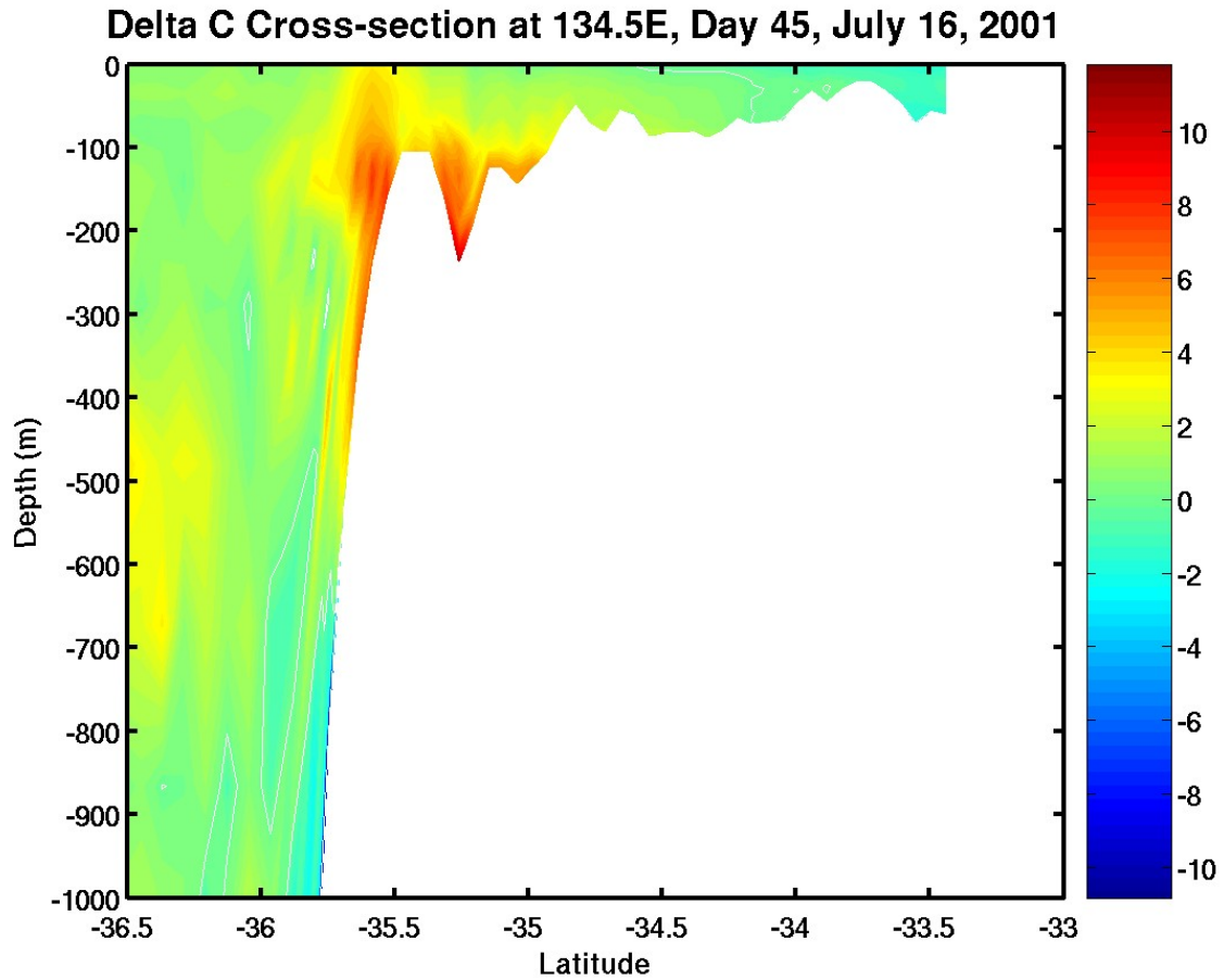
Figure 6.3c. Cross-section of sound speed change ( \text{m s}^{-1} ) in the eastern Great Australian Bight ( 134.5^\circ\text{E} ) for daily wind Experiment 4 on day 45, July 16, 2001. Sound speed change is the difference in sound speed between Day 0 and the current day.
