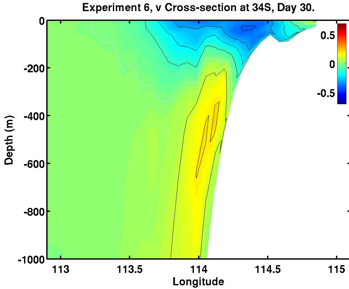
Figure 4.21b. Cross-section of meridional velocity component ( \text{m s}^{-1} ) near Cape Leeuwin ( 34^{\circ}\text{S} ) for Experiment 6 on day 30. Red is equatorward (north) and blue is poleward (south). The white contour is zero.
