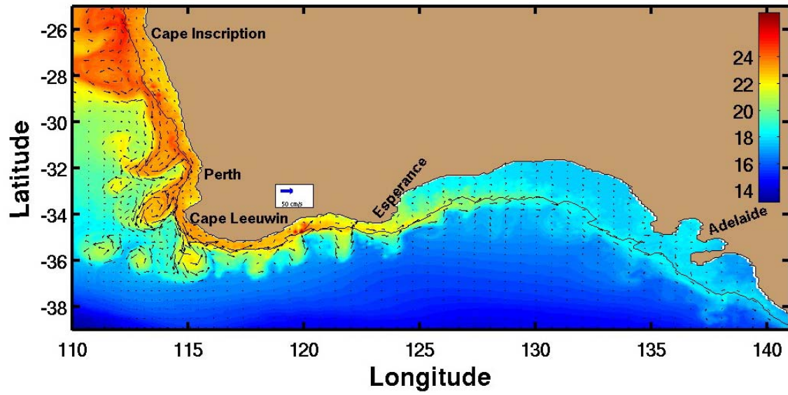
Figure 4.25. Sea surface temperature (°C) and velocity vectors for Experiment 6 on day 75.
