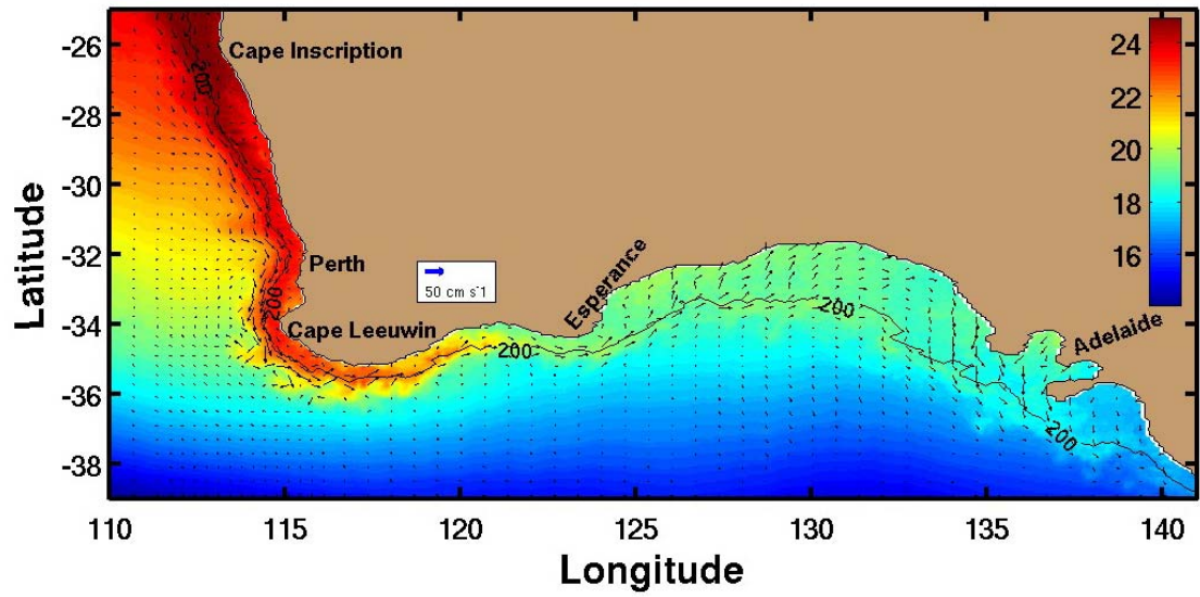
Figure 5.11a. Sea surface temperature ( ^{\circ}\text{C} ) and velocity vectors for daily wind Experiment 3 on day 30, December 31, 2000.
