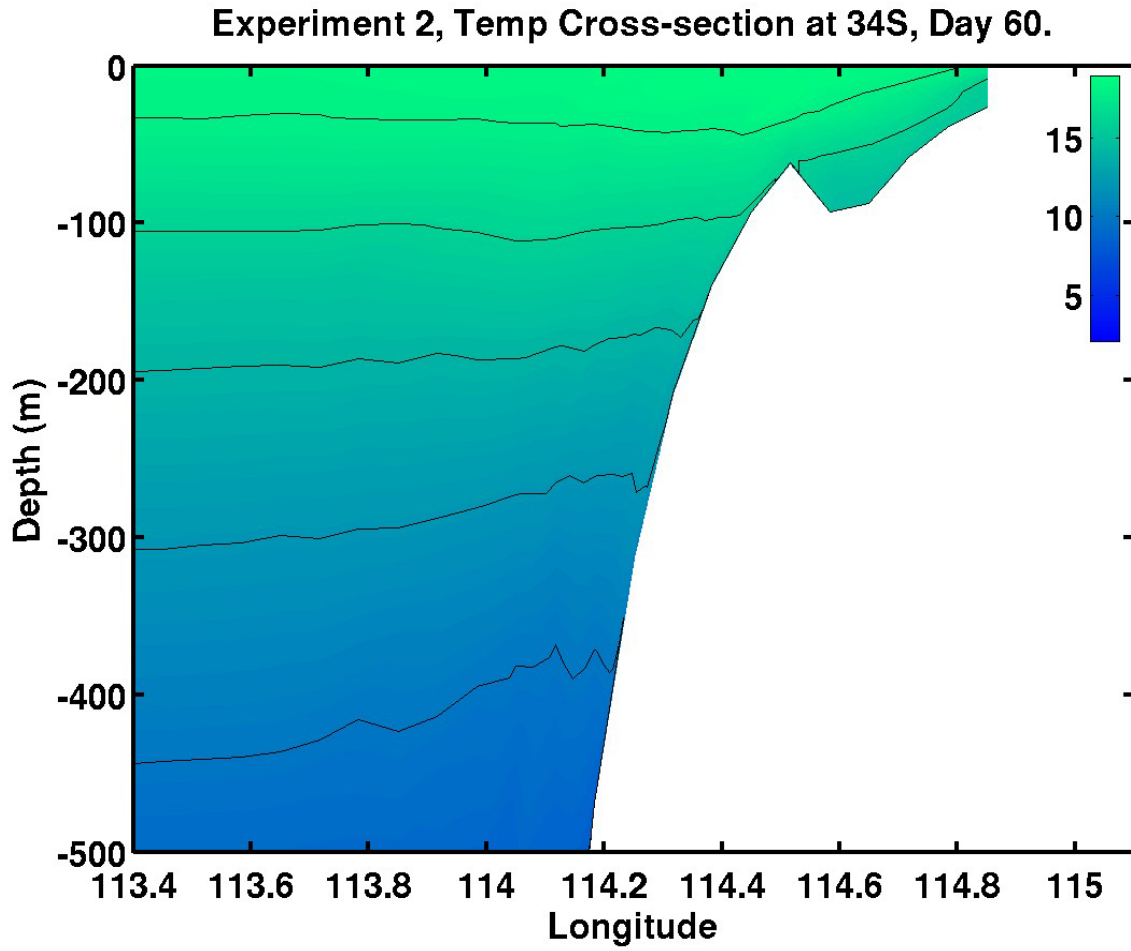
Figure 4.6e. Cross-section of temperature ( ^{\circ}\text{C} ) along an east-west transect near Cape Leeuwin ( 34^{\circ}\text{S} ) for Experiment 2 on day 60.
