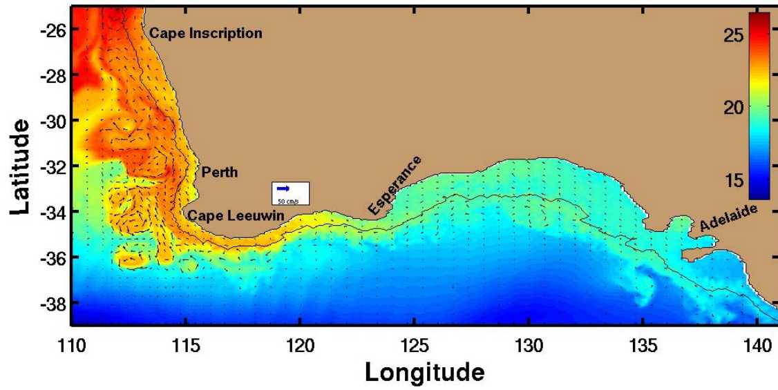
Figure 4.30. Sea surface temperature ( ^{\circ}\text{C} ) and velocity vectors for Experiment 7 on day 81.
