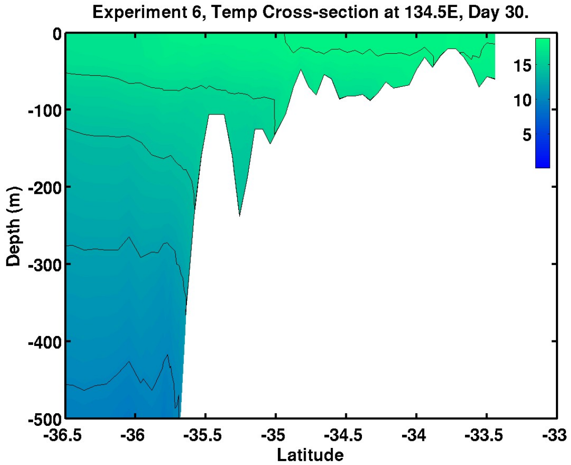
Figure 4.21j. Cross-section of temperature ( ^{\circ}\text{C} ) along an north-south transect in the eastern Great Australian Bight ( 134.5^{\circ}\text{E} ) for Experiment 6 on day 30.
