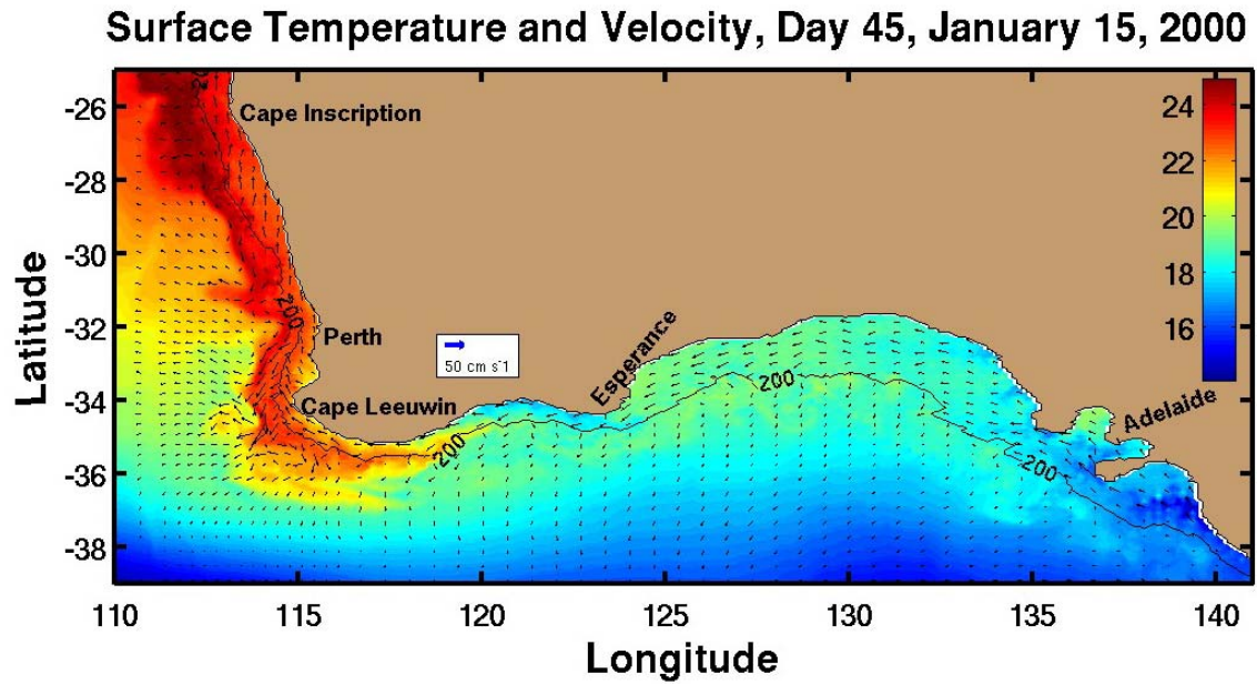
Figure 6.4a. Sea surface temperature ( ^{\circ}\text{C} ) and velocity vectors for daily wind Experiment 3 on day 45, January 15, 2000.
