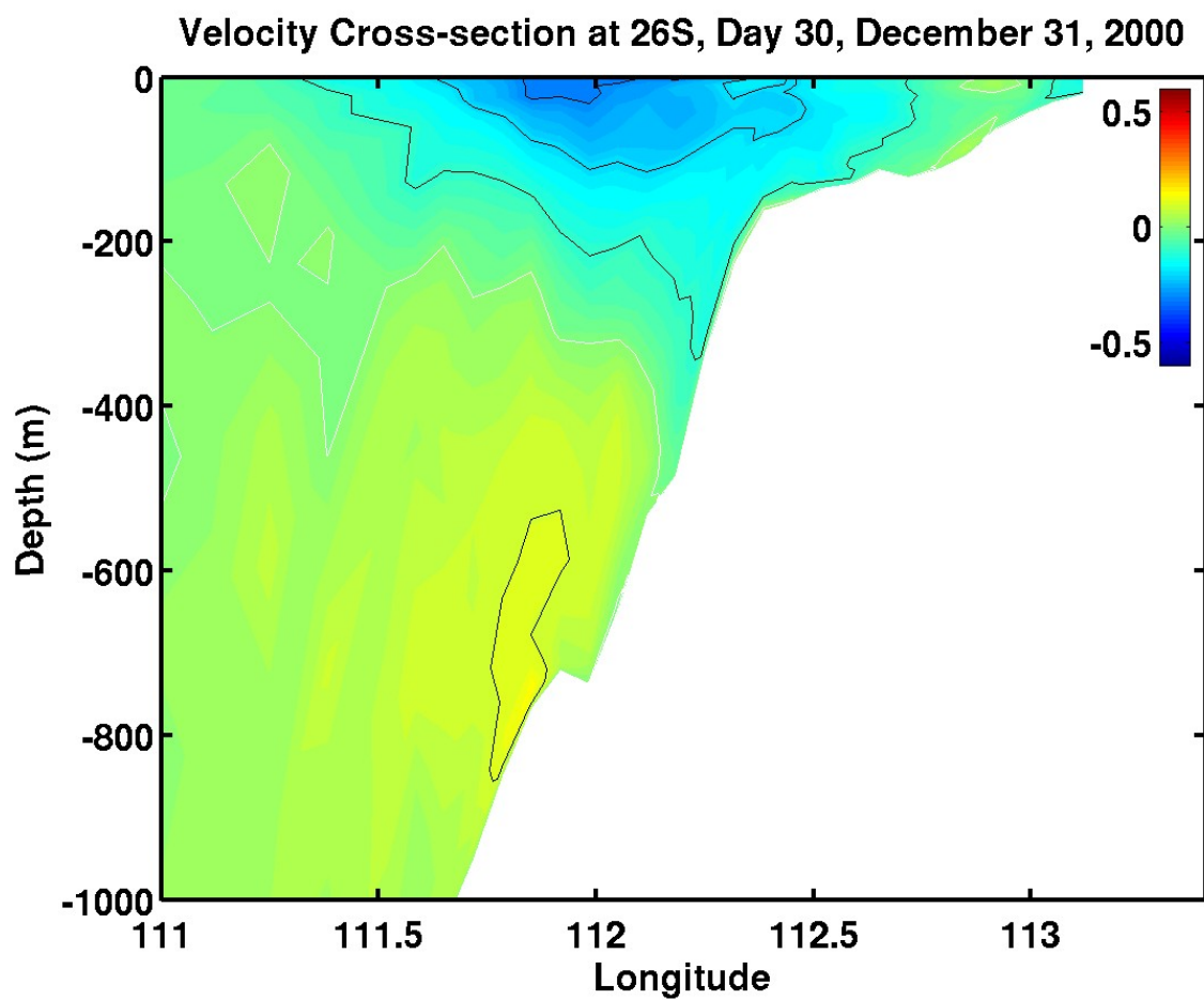
Figure 5.11b. Cross-section of meridional velocity component ( \text{m s}^{-1} ) at 26^{\circ}\text{S} for daily wind Experiment 3 on day 30, December 31, 2000. Red is equatorward (north) and blue is poleward (south). The white contour is zero.
