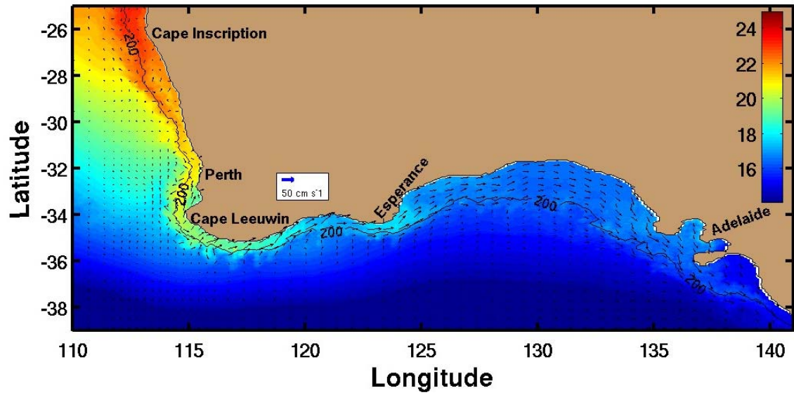
Figure 5.5. Sea surface temperature (°C) and velocity vectors for daily wind Experiment 2 on day 20, June 21, 1981.
