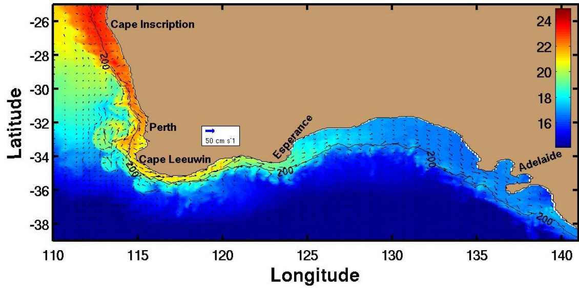
Figure 5.8a. Sea surface temperature (°C) and velocity vectors for daily wind Experiment 2 on day 60, July 31, 1981.
