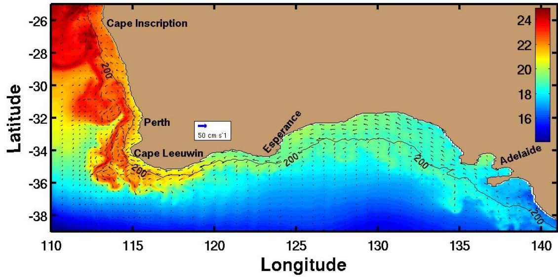
Figure 5.4a. Sea surface temperature (°C) and velocity vectors for daily wind Experiment 1 on day 60, January 30, 1981.
