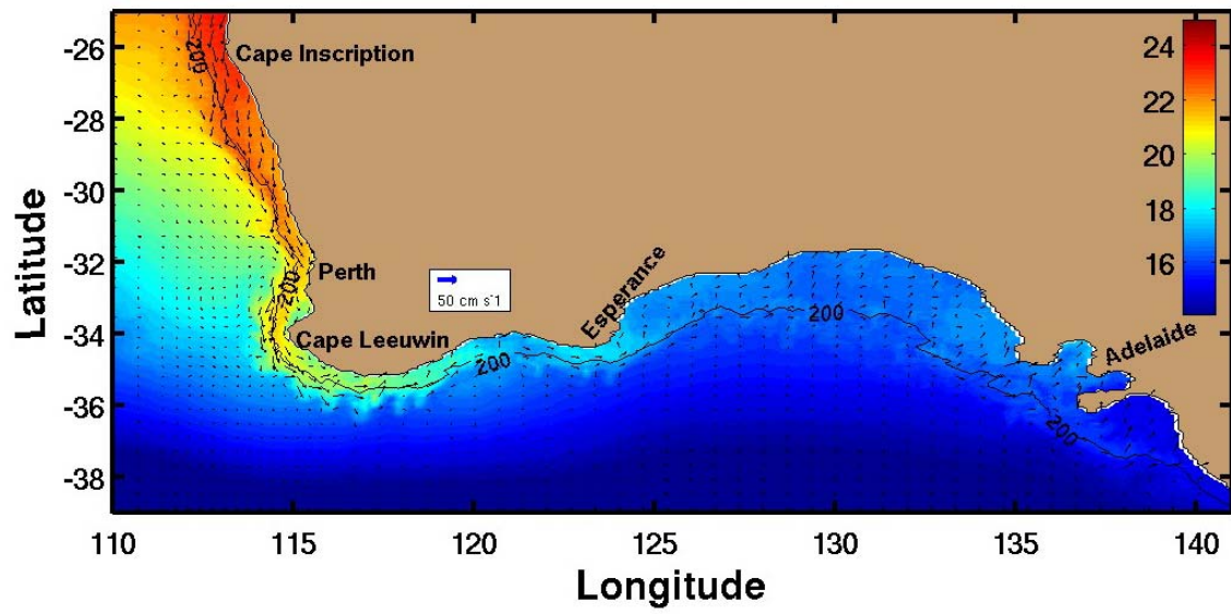
Figure 5.17a. Sea surface temperature (°C) and velocity vectors for daily wind Experiment 4 on day 20, June 21, 2001.
