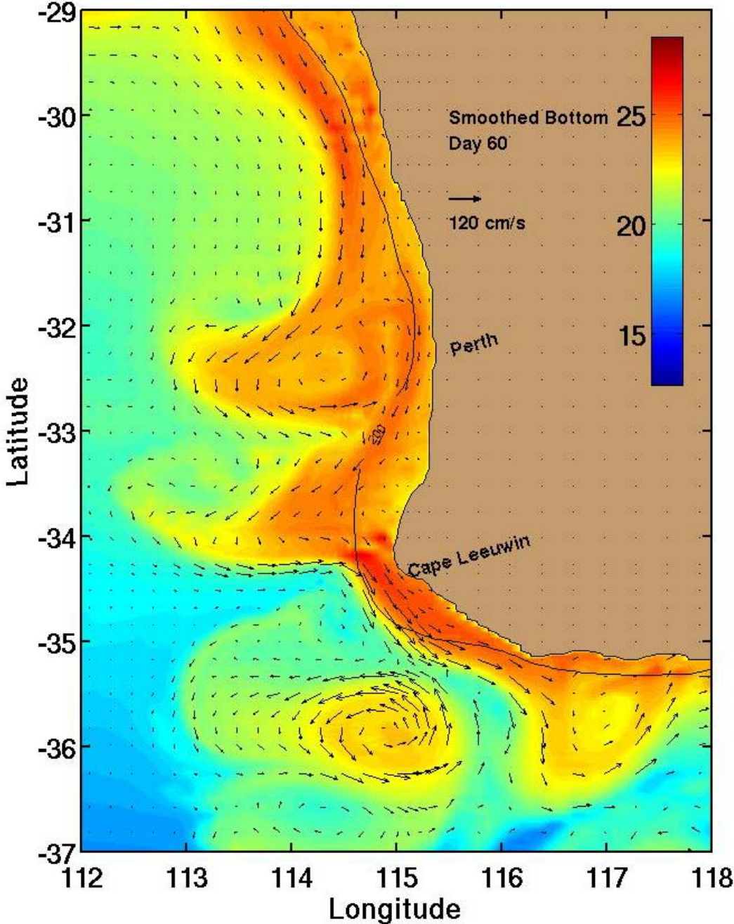
Figure 3.2c. Surface velocity vectors and color-shaded sea surface temperature for day 60 for the model run with topography. The solid line depicts the 200 m isobath, the approximate location of the shelf break.
