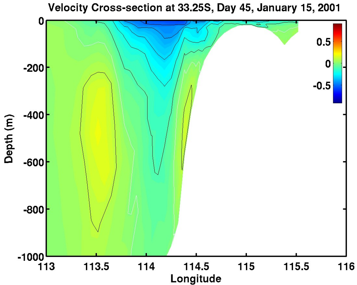
Figure 5.12c. Cross-section of meridional velocity component ( \text{m s}^{-1} ) just north of Cape Leeuwin at 33.25^{\circ}\text{S} for daily wind Experiment 3 on day 45, January 15, 2001. Red is equatorward (north) and blue is poleward (south). The white contour is zero.
