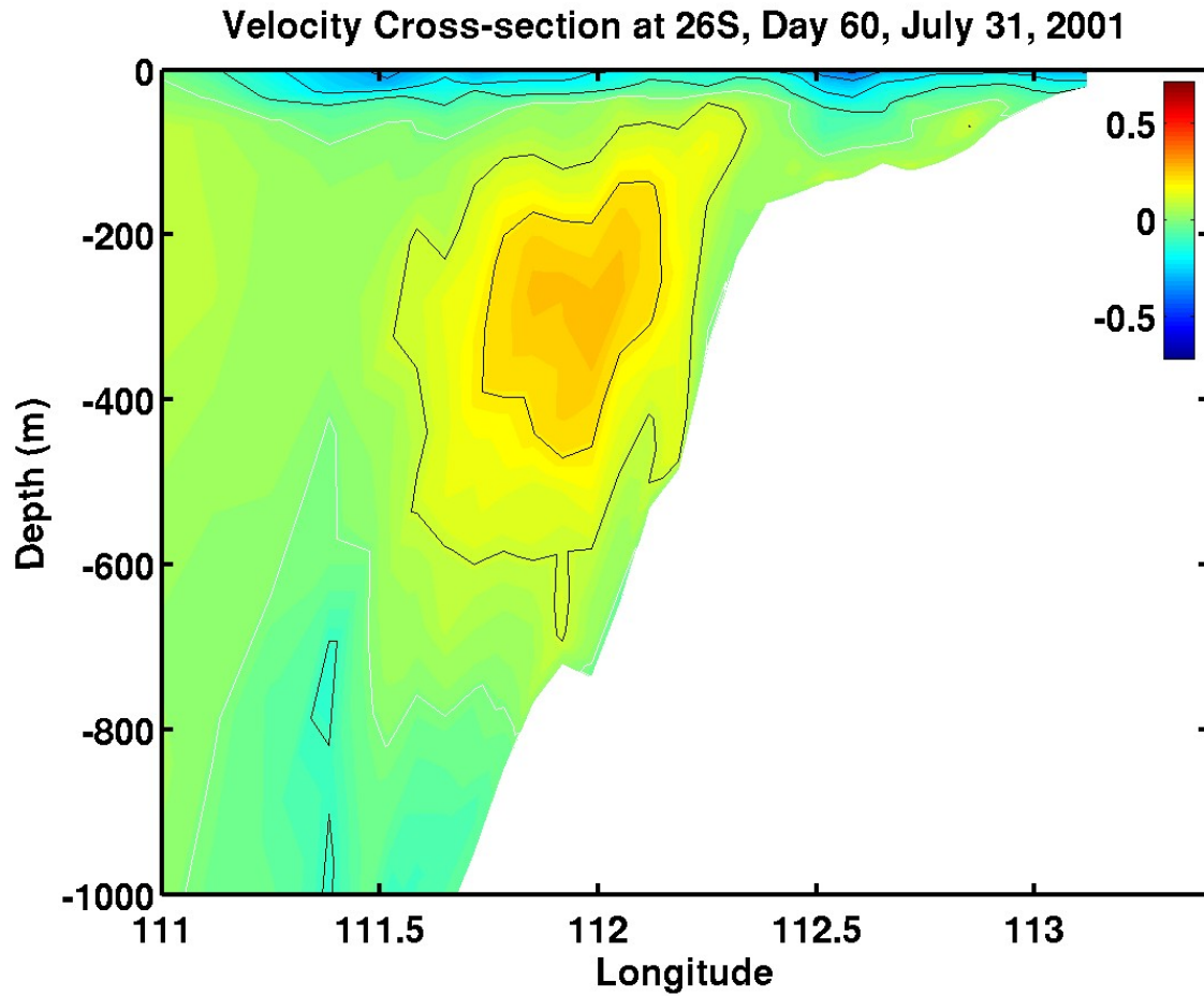
Figure 5.20b. Cross-section of meridional velocity component ( \text{m s}^{-1} ) at 26^{\circ}\text{S} for daily wind Experiment 4 on day 60, July 31, 2001. Red is equatorward (north) and blue is poleward (south). The white contour is zero.
