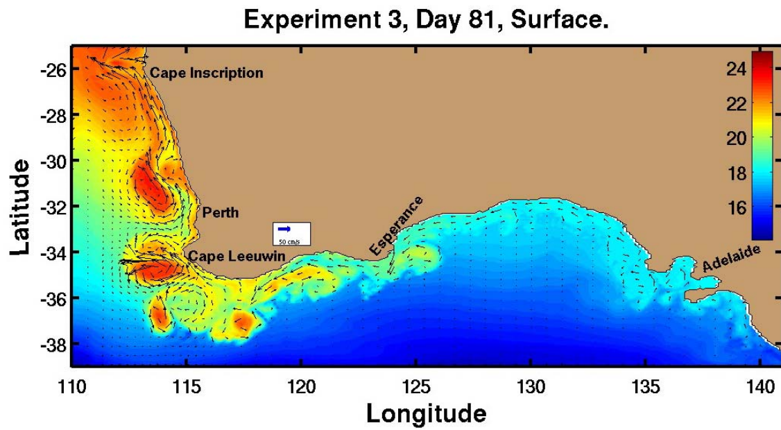
Figure 4.10. Sea surface temperature ( ^{\circ}\text{C} ) and velocity vectors for Experiment 3 on day 81.
