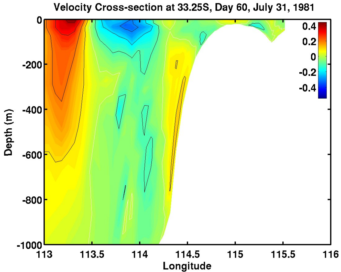
Figure 5.8b. Cross-section of meridional velocity component ( \text{m s}^{-1} ) 33.25^{\circ}\text{S} for daily wind Experiment 2 on day 60, July 31, 1981. Red is equatorward (north) and blue is poleward (south). The white contour is zero.
