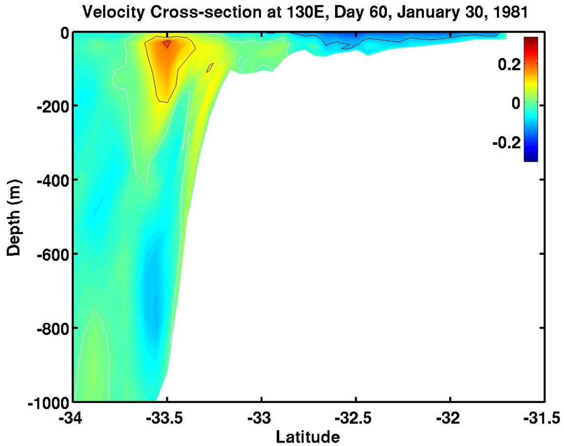
Figure 5.4c. Cross-section of zonal velocity component ( \text{m s}^{-1} ) in the Great Australian Bight ( 130^{\circ}\text{E} ) for daily wind Experiment 1 on day 60, January 30, 1981. Red is eastward and blue is westward. The white contour is zero.
