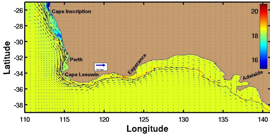
Figure 4.6a. Sea surface temperature ( ^{\circ}\text{C} ) and velocity vectors for Experiment 2 on day 60.
