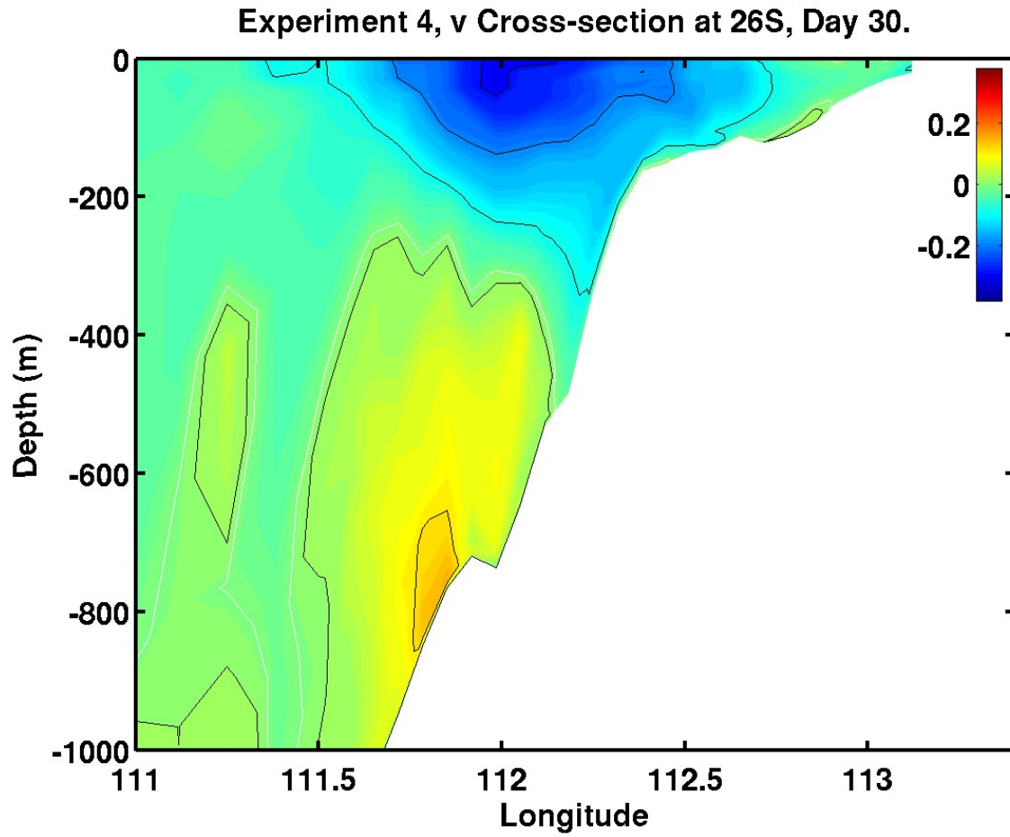
Figure 4.12b. Cross-section of meridional velocity component ( \text{m s}^{-1} ) at 26^{\circ}\text{S} for Experiment 4 on day 30. Red is equatorward (north) and blue is poleward (south). The white contour is zero.
