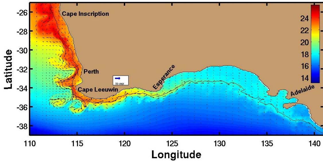
Figure 4.23. Sea surface temperature ( ^{\circ}\text{C} ) and velocity vectors for Experiment 6 on day 51.
