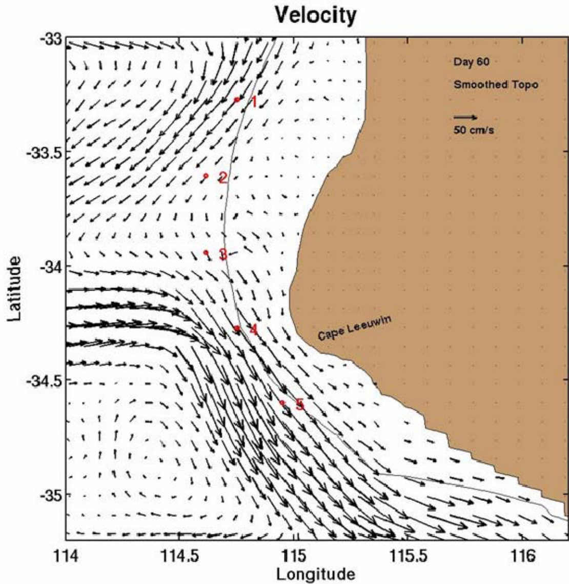
Figure 3.4c. Surface velocity vectors depicting the Leeuwin Current approaching and rounding Cape Leeuwin at day 60 for the smoothed topography model run. The red circles which are numbered in red show the locations of the analysis points used in the Lagrangian dynamical analysis. The solid line depicts the 200 m isobath, the approximate location of the shelf break.
