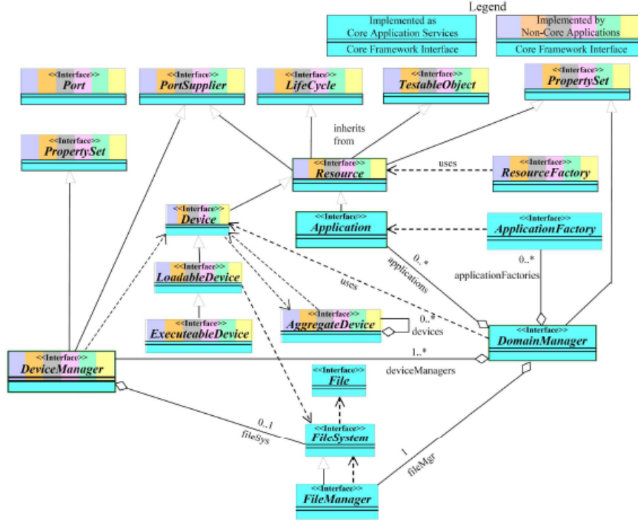
Figure 10. SCA Core Framework IDL relationships (From [17]).
