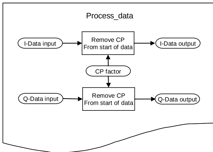
Figure 36. Functional description of component cpRem_802_16 .
