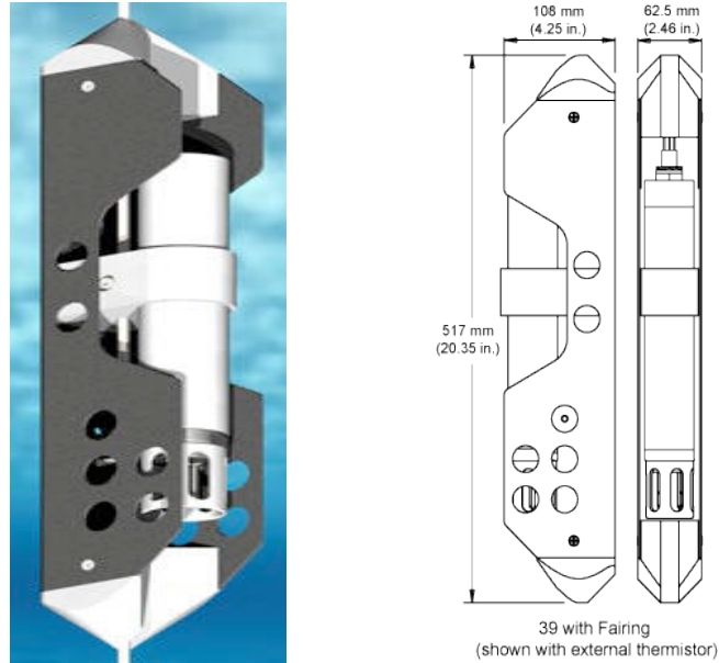
Figure 10. SBE39 Temperature and Pressure Recorder recorded the temperature and pressure every 15 seconds at 15 different depths. (From www.seabird.com )
