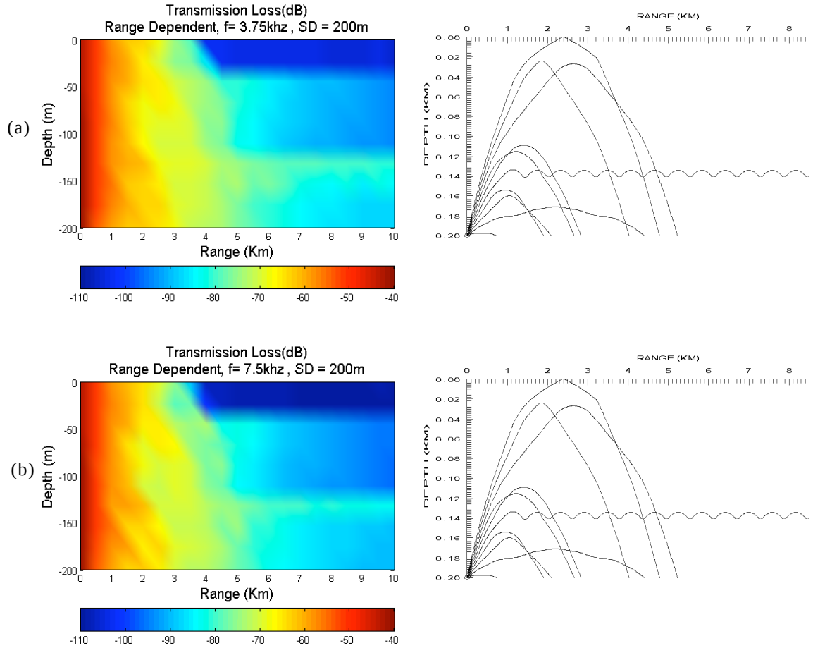
Figure 43. Surface Reflection and Sound Channel at depth of about 140 meters at source depth of 200 m of (a) f = 3.75\text{kHz} , (b) f = 7.5\text{kHz} .
