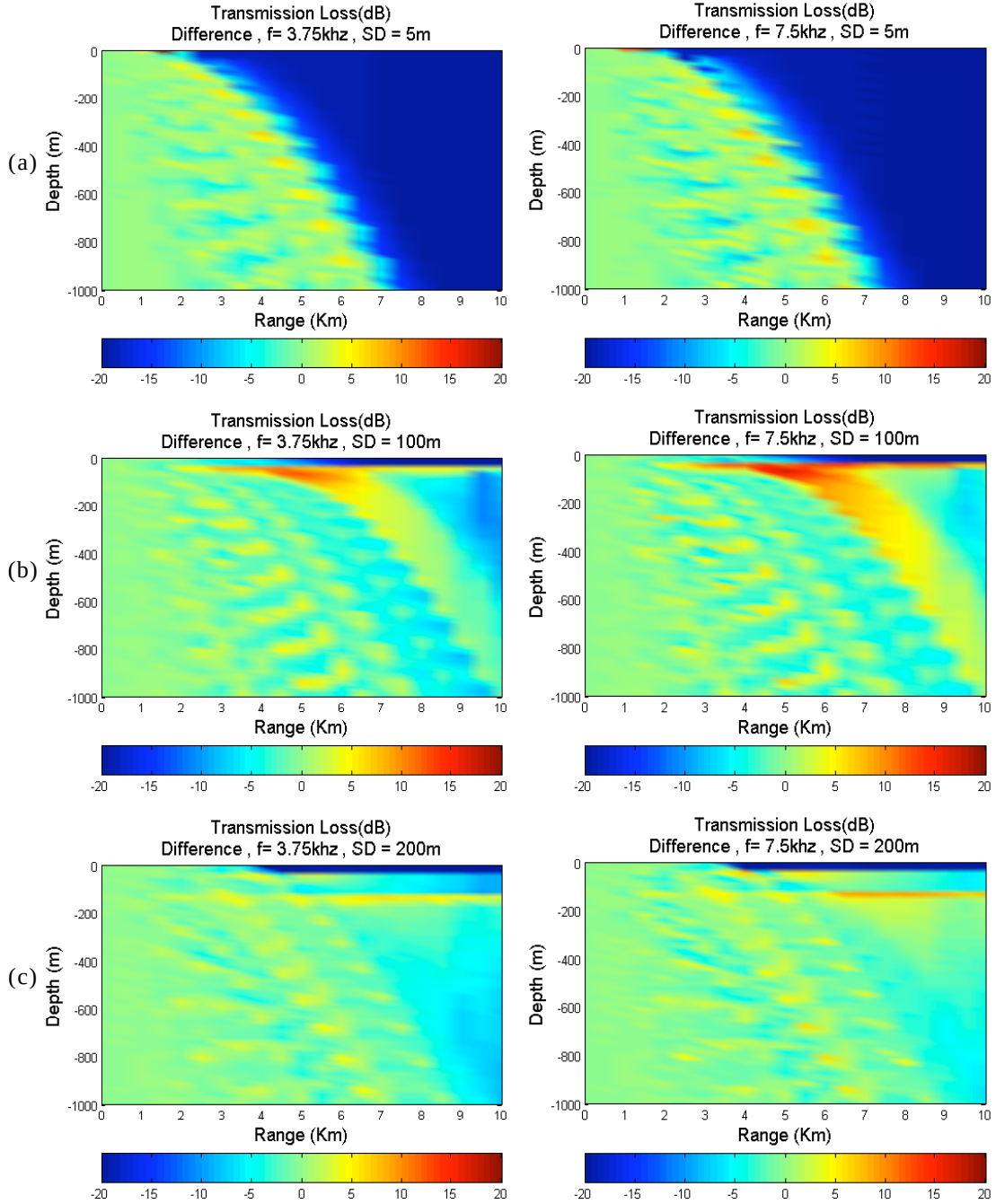
Figure 48. Transmission Loss difference of f = 3.75 kHz (left) and f = 7.5 kHz (right) at different source depths of (a) 5, (b) 100, and (c) 200 meters.
