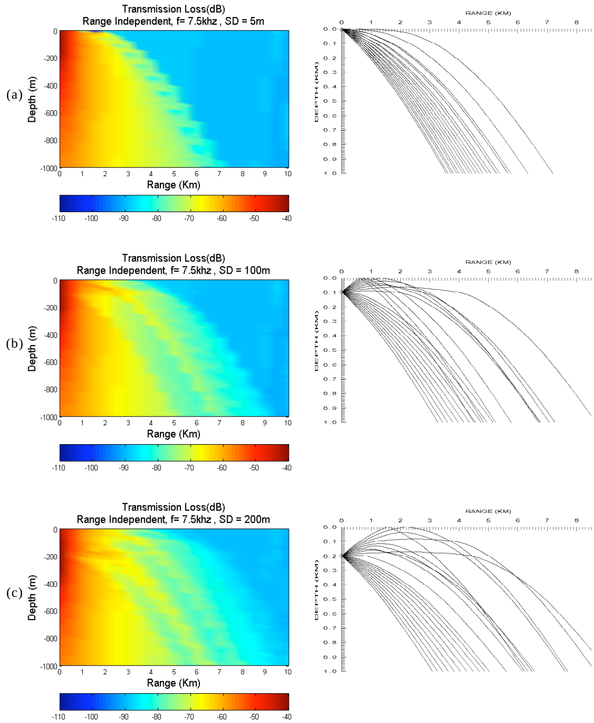
Figure 46. Transmission Loss (left) and Ray trace (right) of Range-Independent cases of f = 7.5 \text{ kHz} at different source depths of (a) 5, (b) 100, and (c) 200 meters.
