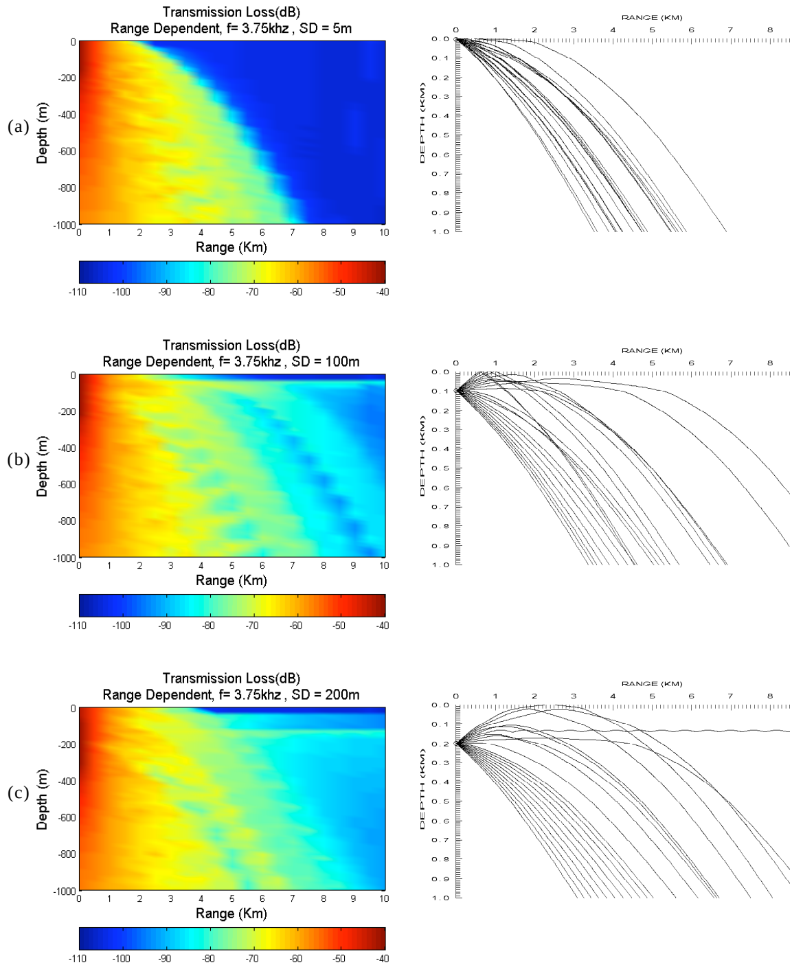
Figure 40. Transmission Loss (left) and Ray trace (right) of Range-Dependent cases of f = 3.75 \text{ kHz} at different source depths of (a) 5, (b) 100, and (c) 200 meters.
