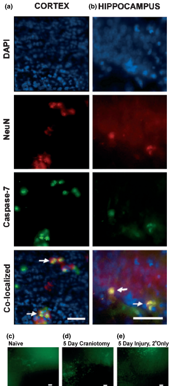
Fig. 6 Traumatic brain injury (TBI) activation of caspase 7 in neurons in the cortex and hippocampus. Caspase 7 expression induced in cortical (a) and hippocampal (b) neurons after TBI was examined using immunohistochemical techniques on 40- \mu m brain tissue sections. Chromatin was visualized with DAPI, neurons with the neuron-specific antibody anti-neuronal nuclei (NeuN) (red) and caspase 7 with a cleaved anti-caspase 7 antibody (green) with colocalization resulting in yellow and orange (arrows). Photomicrographs are at 400x; scale bars, 20 \mu m. Controls for caspase 7 expression were examined on 40- \mu m brain tissue sections of naïve (c), 5-day craniotomy (d) and 5-day injured tissue (secondary antibody only) (e). No caspase 7 expression was evident and only typical background manifestations were observed. Photomicrographs are at 200x; scale bars, 20 \mu m.
