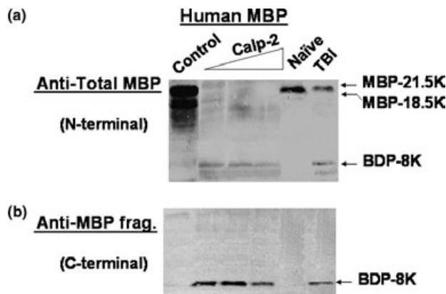
Fig. 8 In vitro proteolysis of purified human myelin basic protein (MBP) with calpain. Purified human MBP (18.5 kDa) was digested with calpain-2 in vitro under conditions similar to those described in Fig. 7. MBP (10 ng) was treated with either no protease (control) or with 0.25%, 0.5% and 1% calpain-2 for comparison with the fragmentation pattern observed in vivo at 48 h after TBI and with naive control (20 \mu g brain lysate each). The samples were then analyzed by immunoblots probed with either anti-total MBP (N-terminal) (a) or MBP-fragment-specific monoclonal antibody (b).
