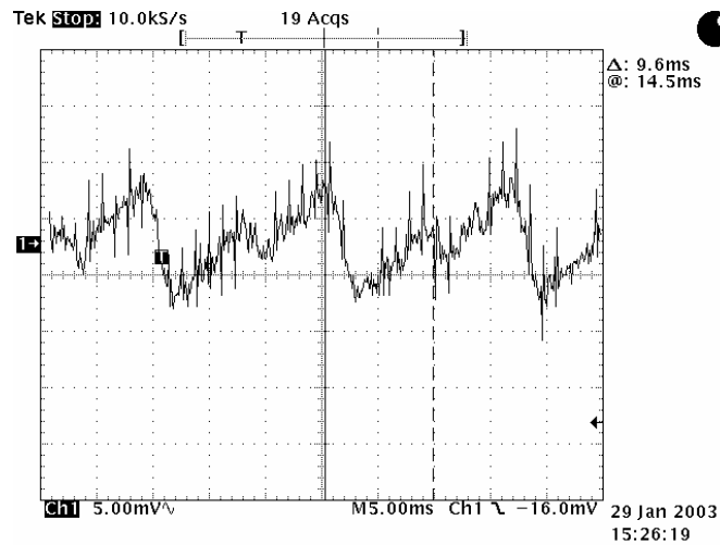
Figure 7. Response of the LCoS projector to a steady test stimulus. Vertical scale: 5 mV/division; Horizontal scale: 5 msec/division.
