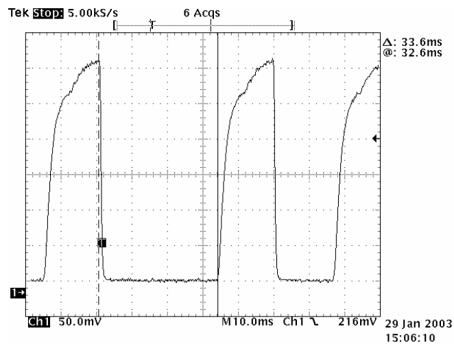
Figure 8. An example of a missed LCoS projector on-frame to a one-frame on / one-frame off flashing test stimulus. Vertical scale: 50 mV/division; Horizontal scale: 10 msec/division.
