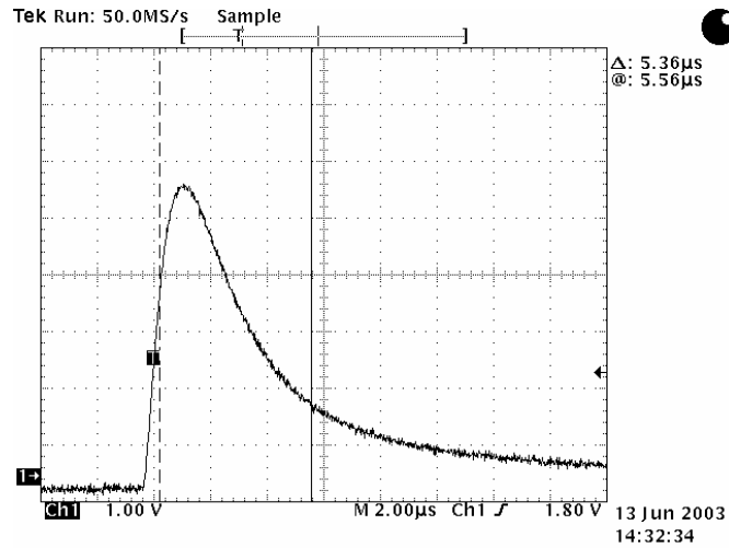
Figure 11. Light output of the CRT projector to a single displayed pixel. Vertical scale: V/division; Horizontal scale: 2 \mu sec/division.
