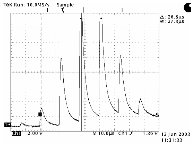
Figure 12. Light output of the CRT projector to a 16.7 msec test stimulus (i.e., a 30 Hz flashing square). Vertical scale: 2 V/division; Horizontal scale: 10 \mu sec/division.
