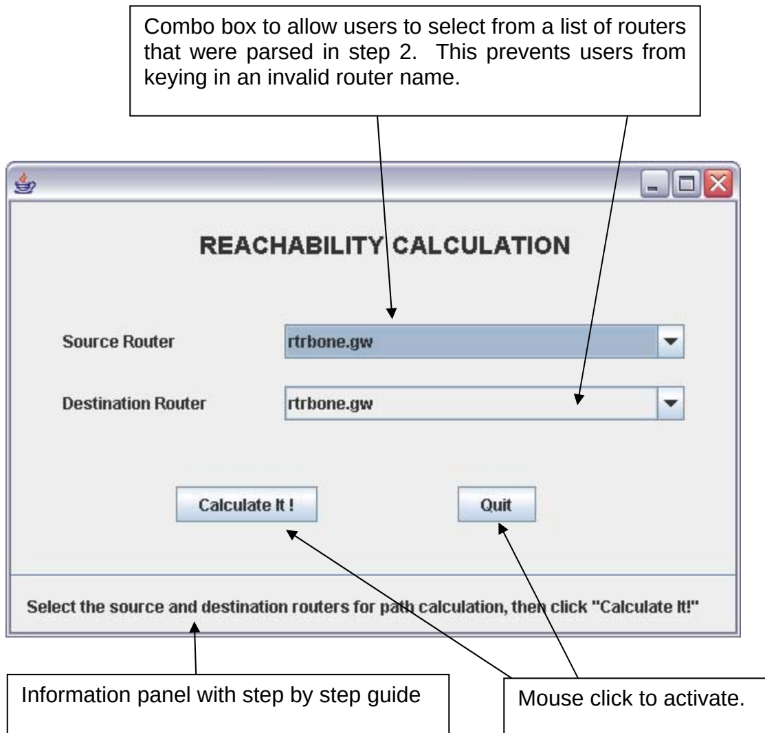
Figure 3. Reachability Calculation Screen
