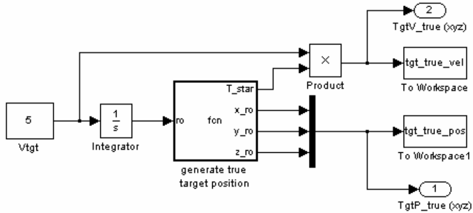
Figure 5. True target vehicle model
