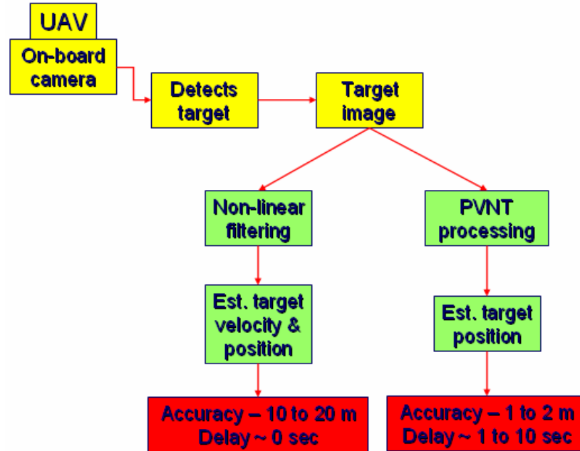
Figure 2. Current architecture
