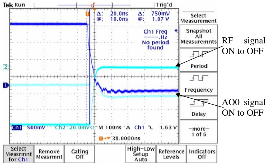
Figure 37. Transmit delay (falling edge) with function generator
