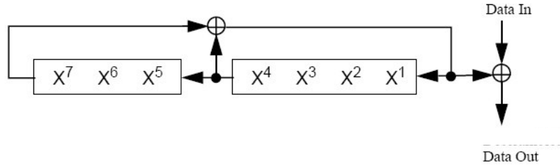
Figure 30. DATA scrambler (from: reference [3], Fig. 113).
