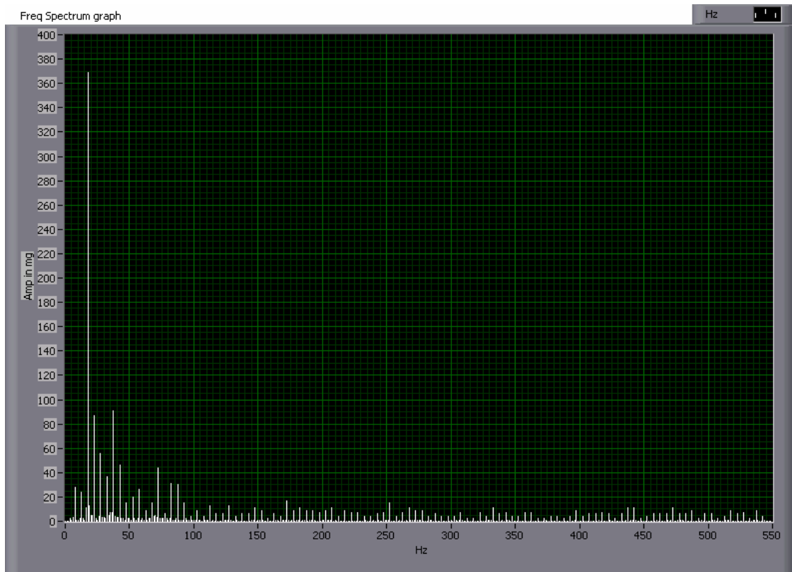
Figure 14. AC unit Vibration Spectrum- Normal Condition
