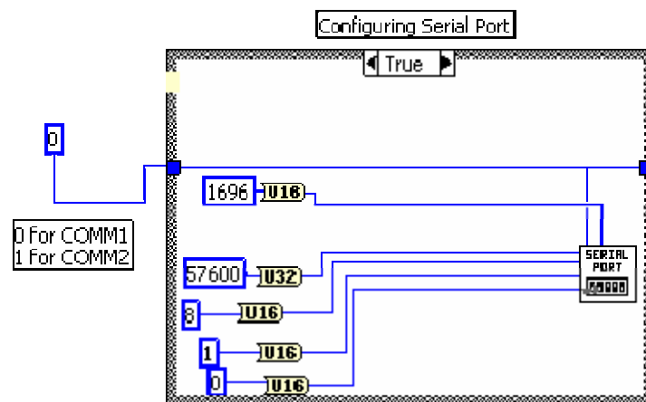
Figure 6. Serial Port Setup
