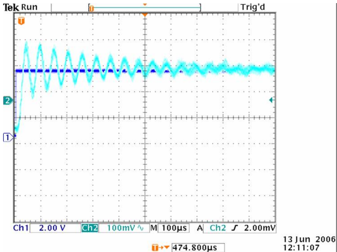
Figure 27. Oscilloscope Display
