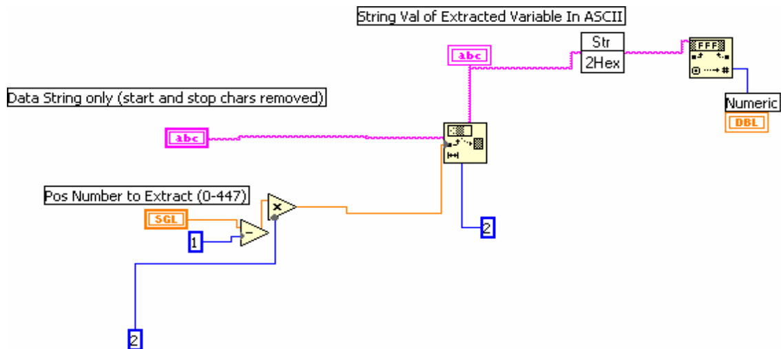
Figure 11. Parse CONV Network
