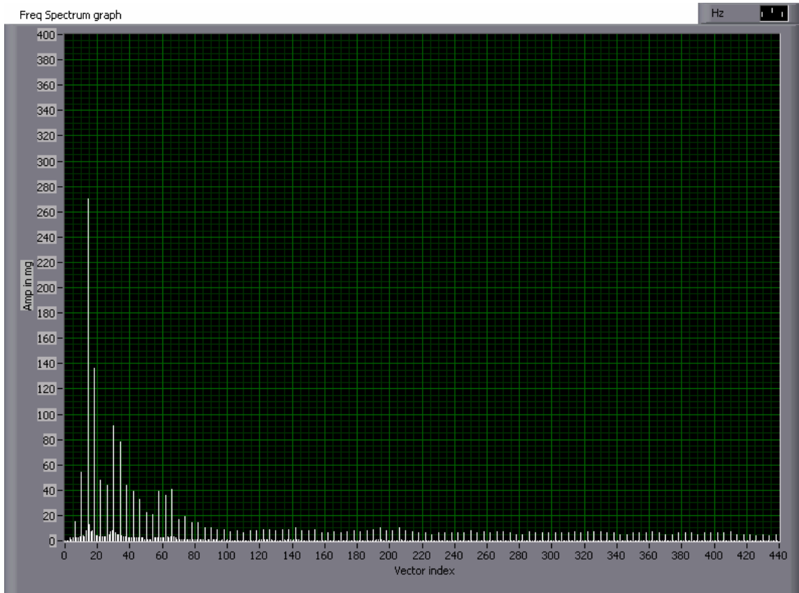
Figure 18. Graph of AC Unit Reference Signal
