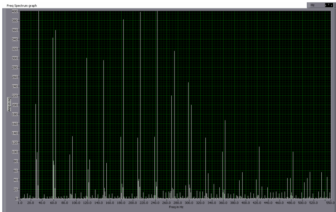
Figure 12. Pump Vibration Spectrum- Normal Condition
