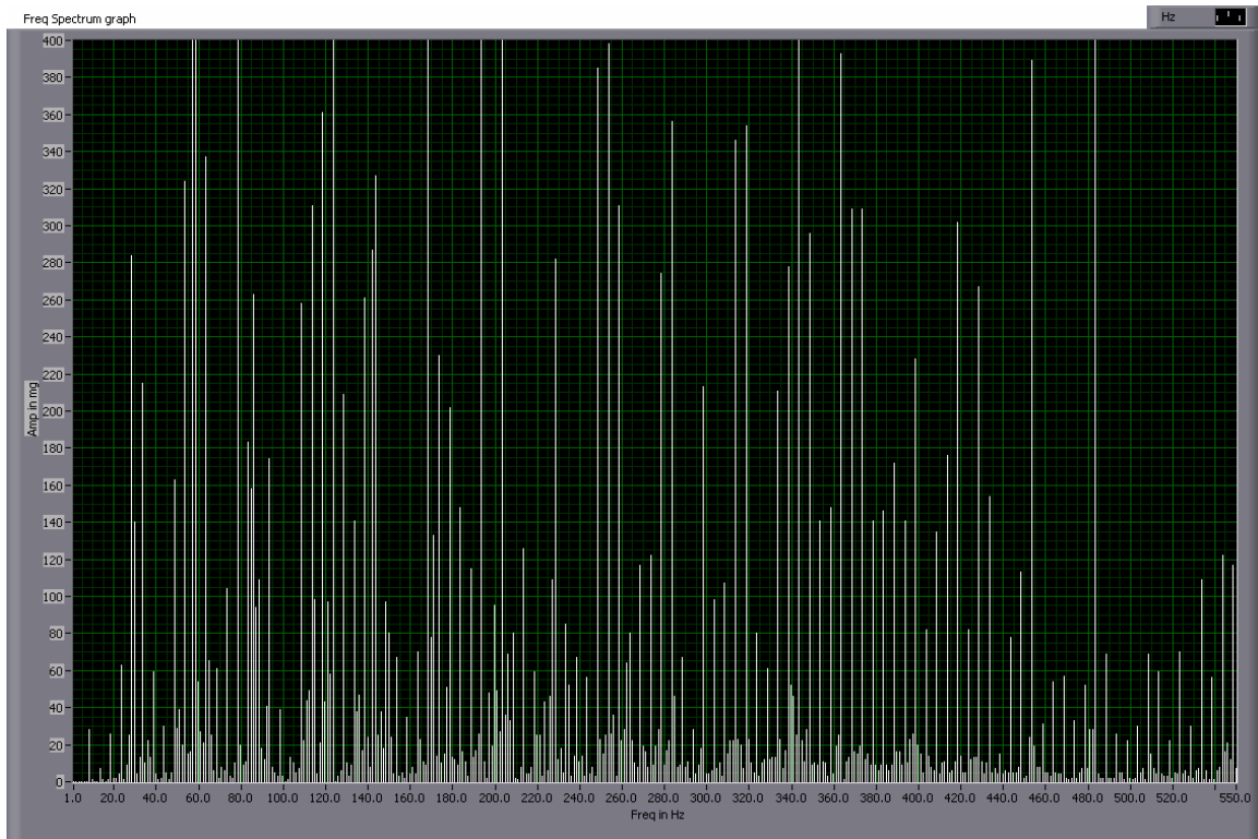
Figure 13. Pump Vibration Spectrum- Damaged Condition (Outlet Blocked)
