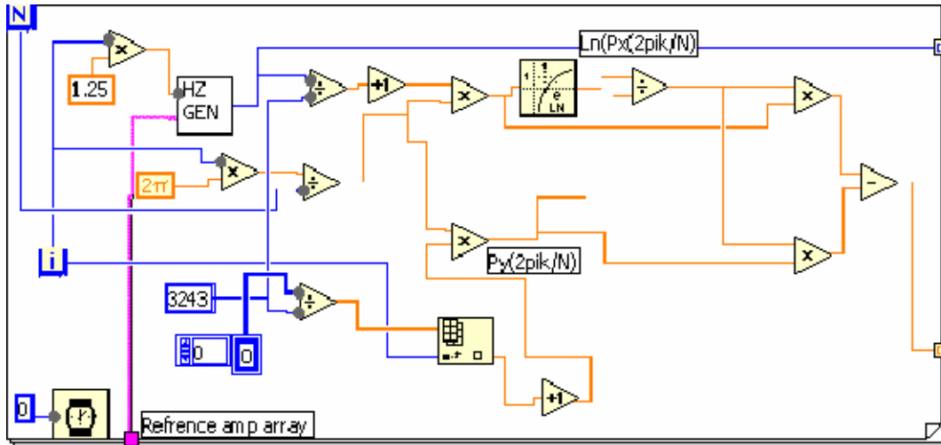
Figure 22. LabView Spectral Distance Network
