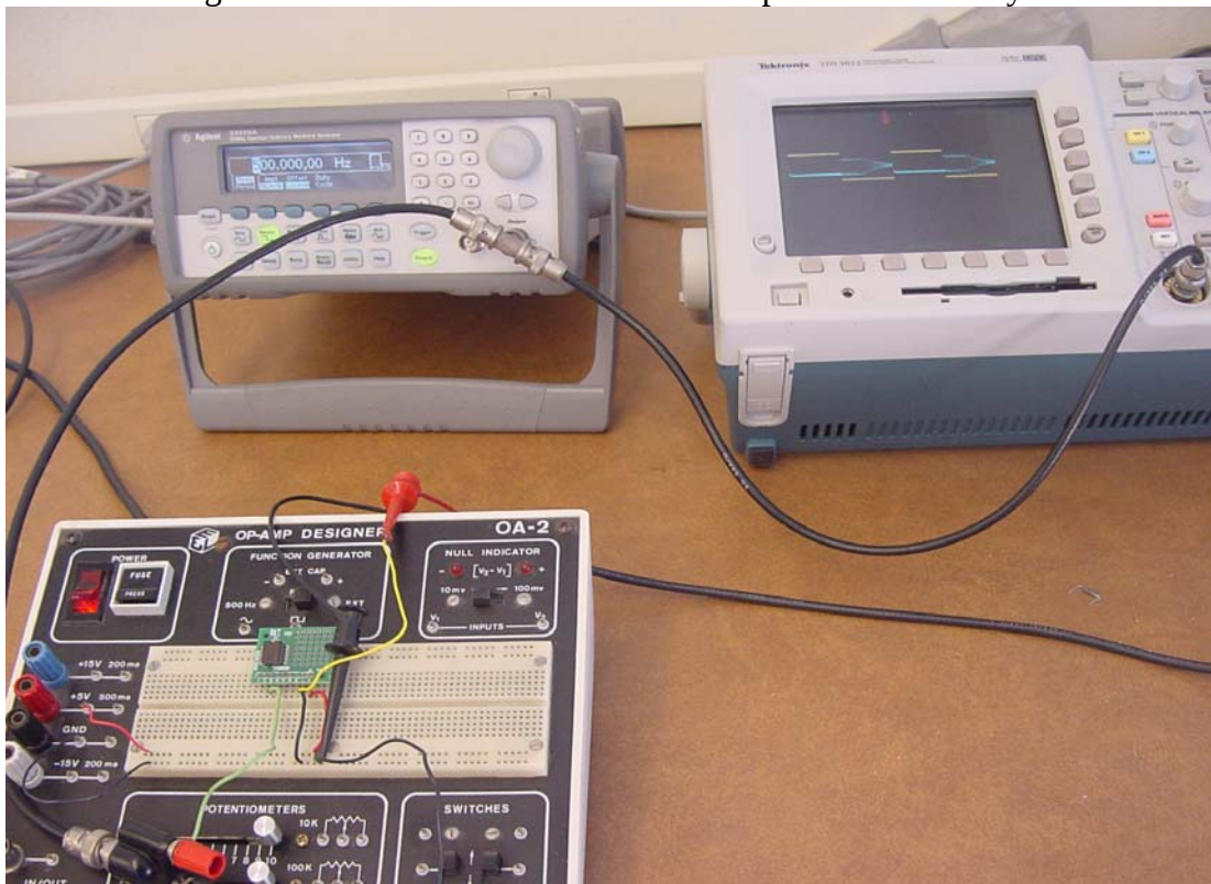
Figure 26. Complete Accelerometer Test Setup
