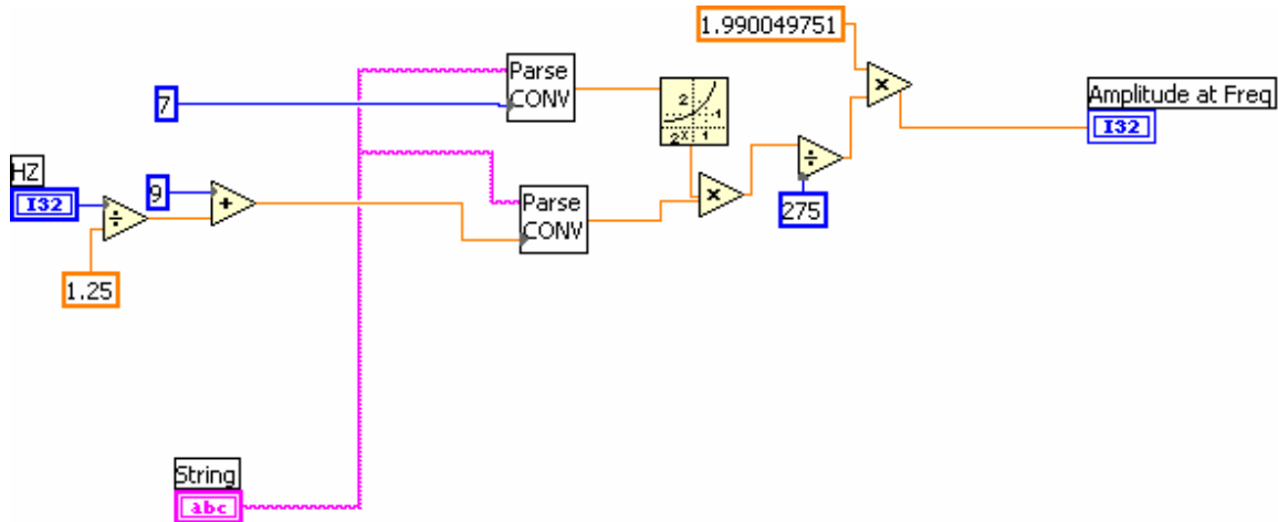
Figure 10. HZ GEN Network
