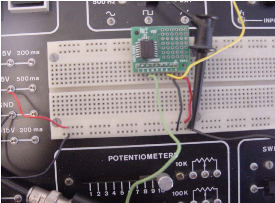
Figure 25. Accelerometer Test Setup Protoboard Only
