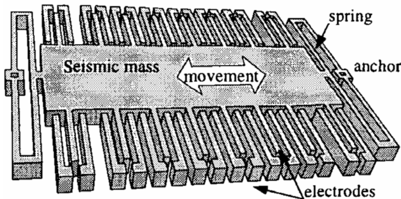
Figure 1. MEMS Vibration Sensor (After Charlot)
