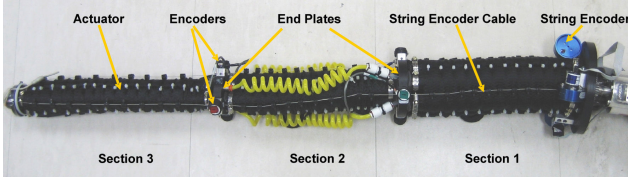
Fig. 1: The OCTARM V.2 robotic manipulator.
