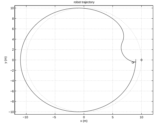
Fig. 2. Trajectories of the Leader ( \diamond , dashed) and the Follower ( \circ , solid).
