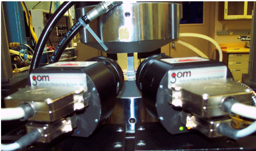
Figure 3: Stereo imaging experimental setup
