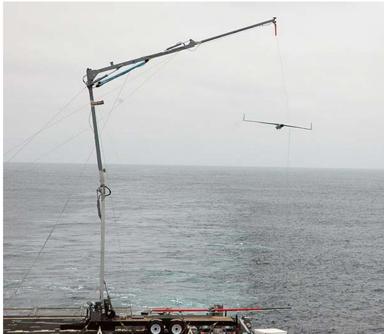
Figure 5. Scan Eagle Recovery System
