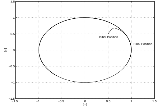
Figure 3: Master System End-Effector Position x_m(t) when the user assist mechanism is enabled (i.e., \gamma = 1 )
