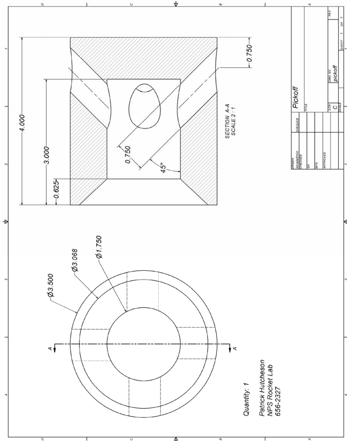
Figure 60. Pickoff
