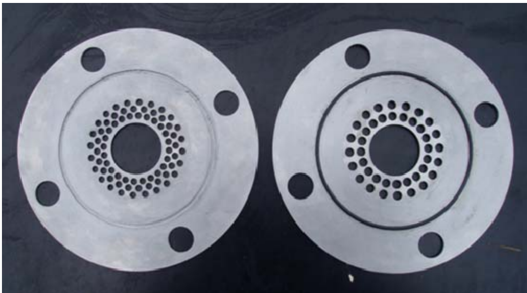
Figure 24. Flow Conditioning Screens
