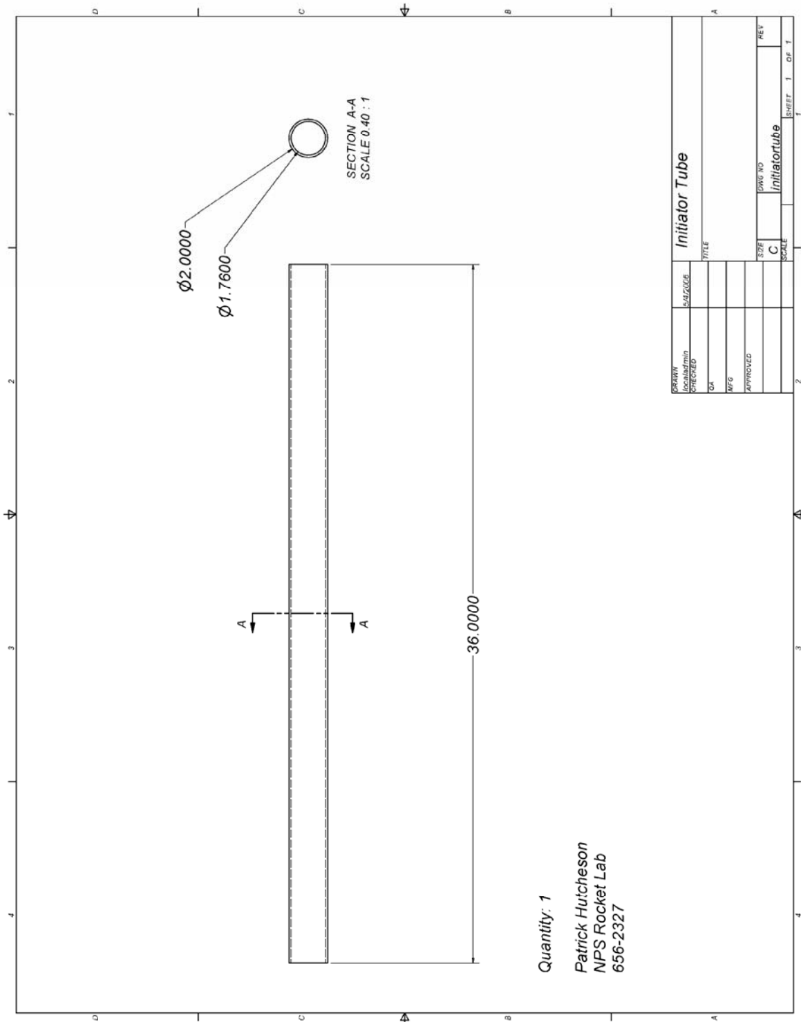
Figure 73. Initiator Tube
