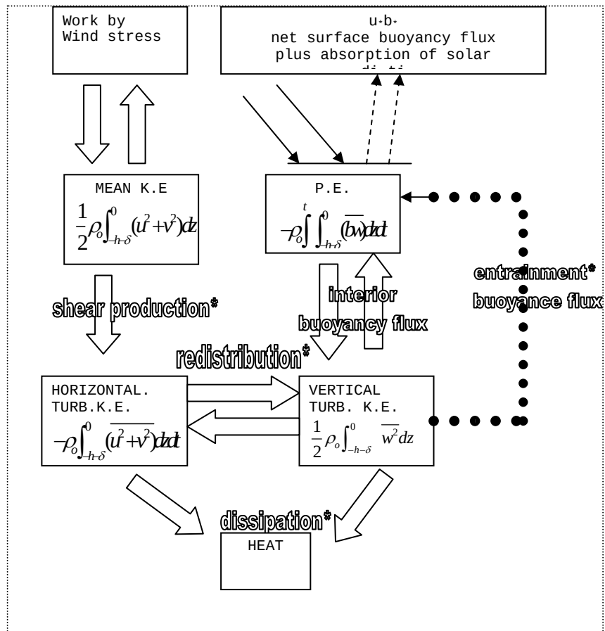
Figure 7. Mechanical energy budget for the ocean mixed layer. Asterisks indicate those processes that must be parameterized to close the system equations (from Garwood, 1977).
