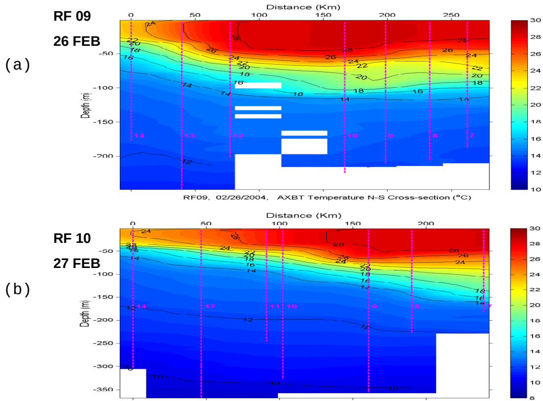
Figure 18. (a) same as Figure 17a; (b) portion of Figure 17b that is close to the location of the AXBT drop track in Figure 17a for RF09.
