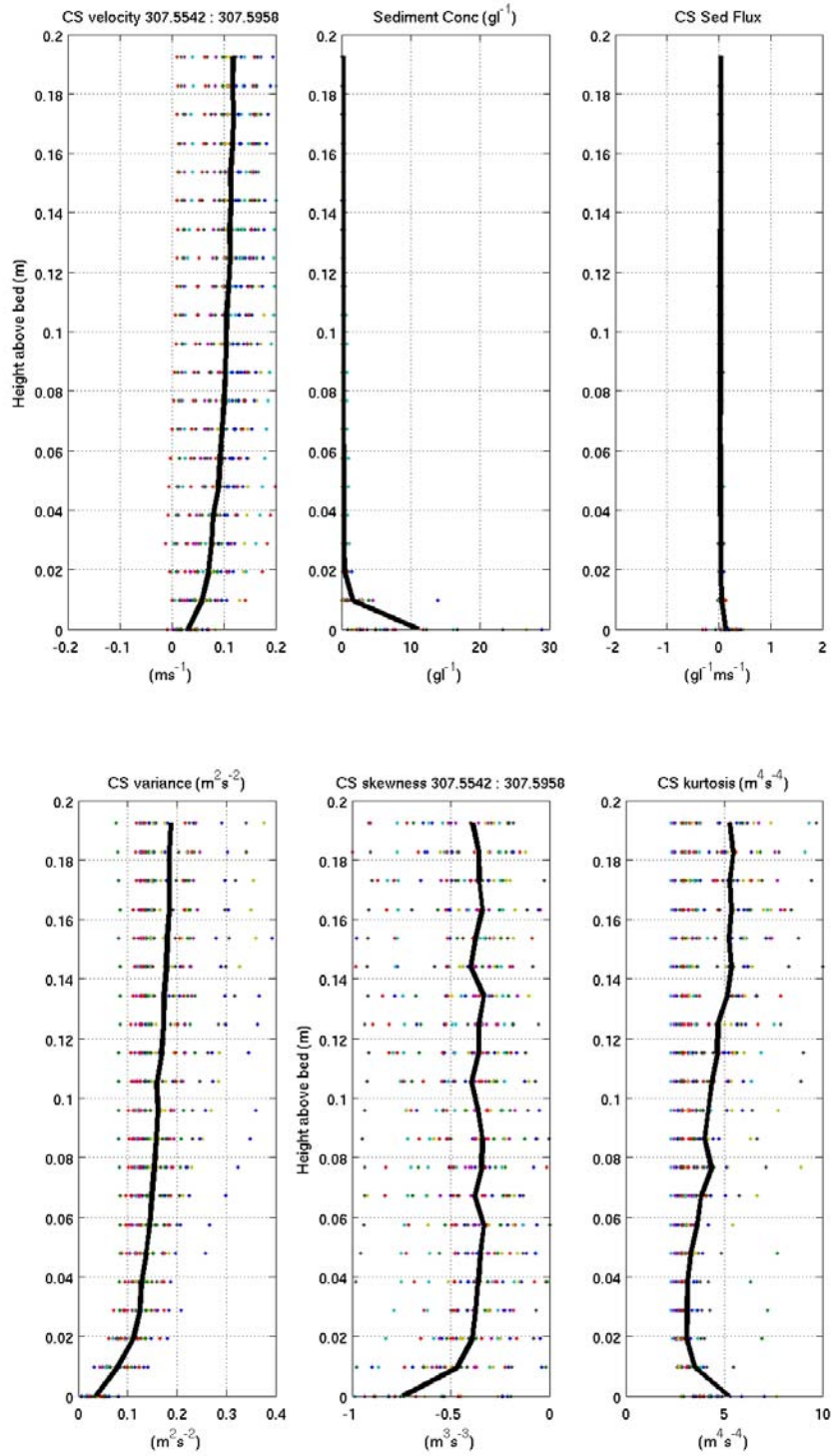
Figure 36. Profiles of Cross-Shore Velocity, Sediment Concentration, Sediment Flux, Variance, Skewness, and Kurtosis for year/day 307.5542.
