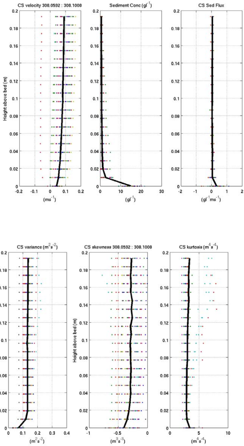
Figure 39. Profiles of Cross-Shore Velocity, Sediment Concentration, Sediment Flux, Variance, Skewness, and Kurtosis for year day 308.0592.
