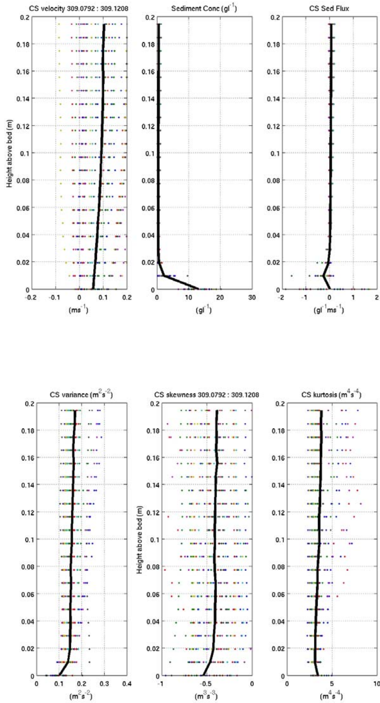
Figure 42. Profiles of Cross-Shore Velocity, Sediment Concentration, Sediment Flux, Variance, Skewness, and Kurtosis for yearday 309.0792.
