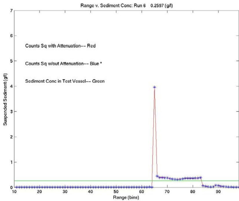
Figure 11. Concentration profiles with /without applied Attenuation Calibration: Run 6.
