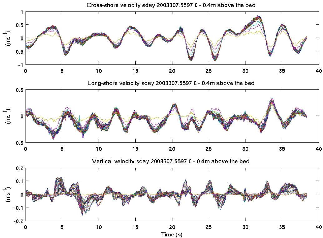
Figure 8. 16 Hz sampled velocity ( u , v , x ) time series recorded by BCDV for bins in the bottom 40 cm above the bed. Each time series is a 35 s time series of the instantaneous velocity returned at 1 cm resolution. Strong gradients in the cross and long shore components are seen in the bottom 2-4 cm, spanning the thin oscillatory boundary layer in the flat, sheet-flow environment seen below the BCDV.
