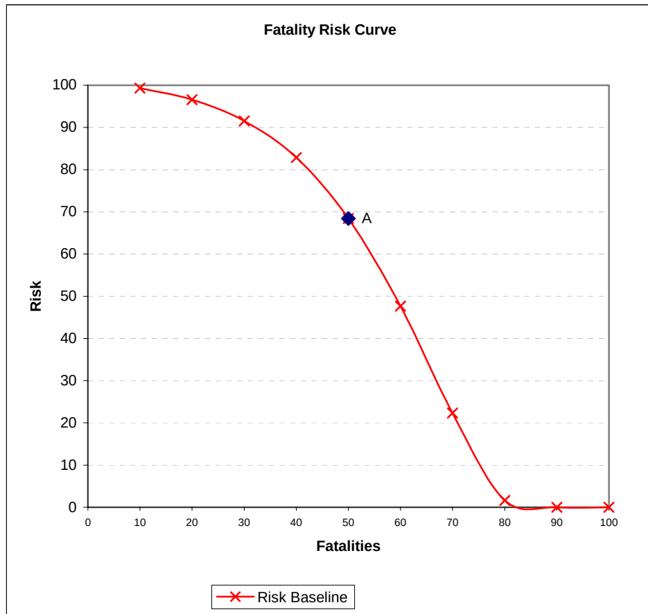
Figure 9 Example Model Baseline Risk Curve
