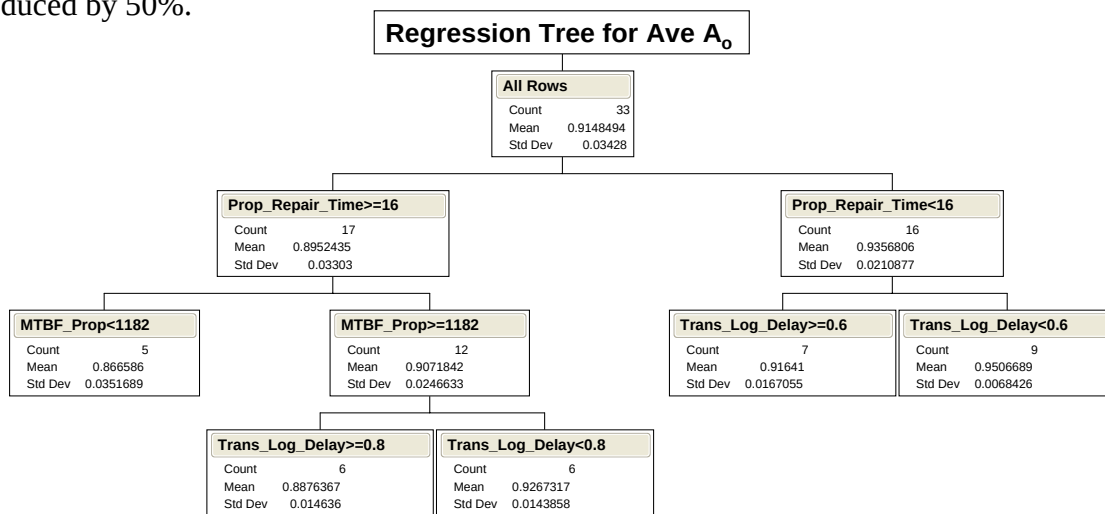
Figure 23 Regression Tree for Average A_0 , Case 4
