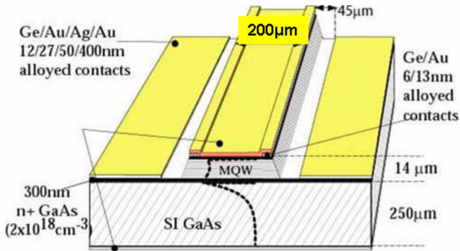
Figure 12. Schematic of 3.4 THz laser (After [20]).
