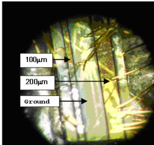
Figure 18. Close-up of the laser.
