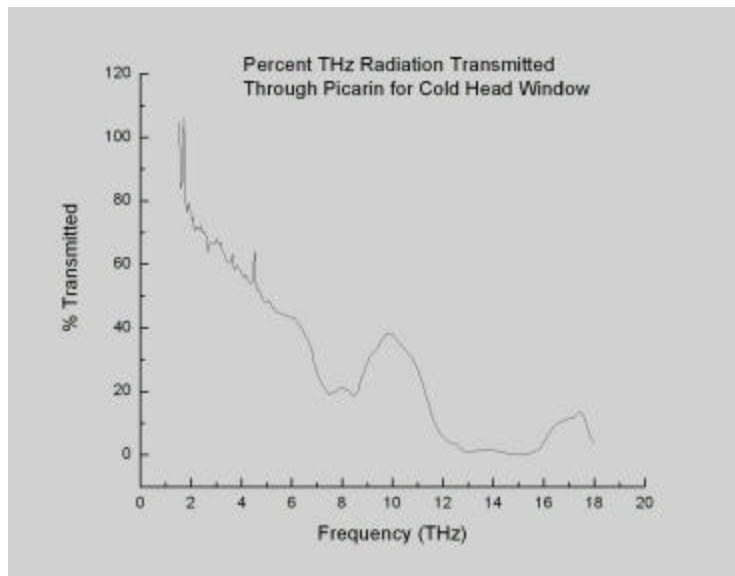
Figure 22. THz transmission through picarin measured with FTIR.
