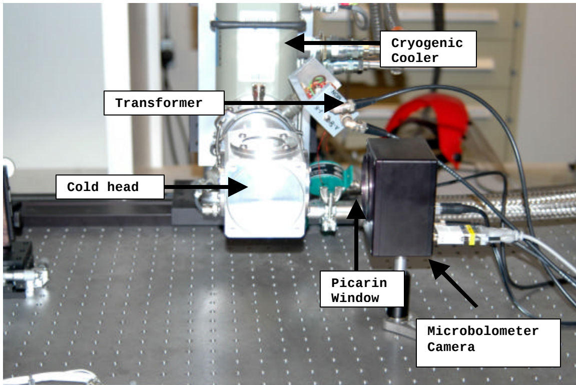
Figure 27. Experiment set-up.
