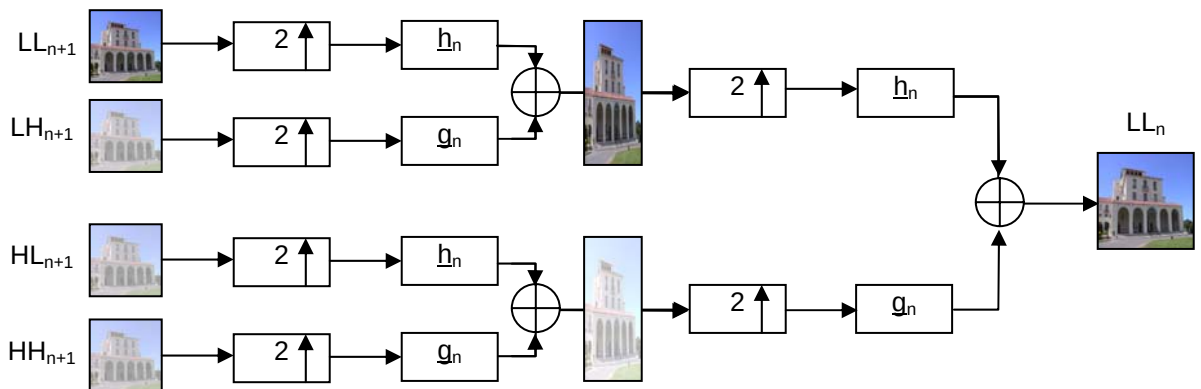
Figure 10. Reconstruction Tree from 4 Subband Images Back to Recover the Original Image. (After: Chow 2004)
