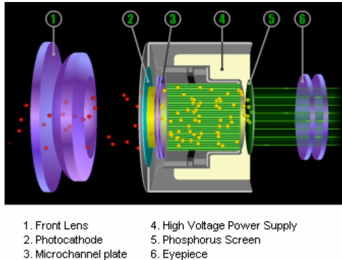
Figure 3. Image Intensifier Internal Construction and Mechanism. (From: American Technologies Network Corporation, Oct 2006)
