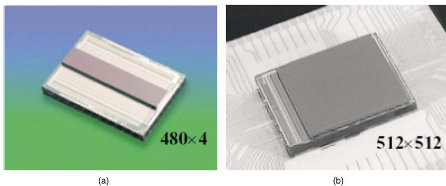
Figure 6. Second-generation PV HgCdTe Detectors, Which are Configured in (a) Parallel Scan with Time Delay Integration (TDI) and (b) Staring (parallel) Sensor Formats (From: Norton, 2002)
