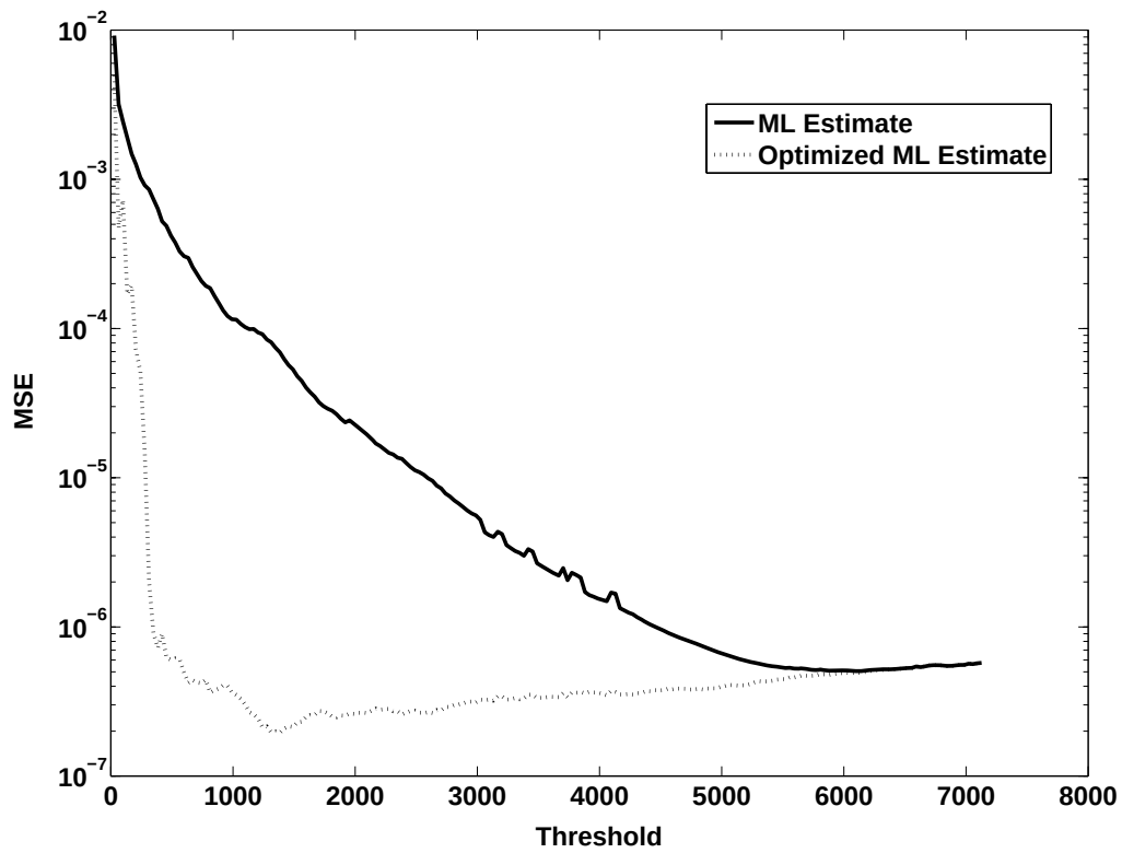
Figure 5.22: MSE of the ML estimator and improved ML estimator with respect to changing the threshold u for the cluster in Figure 5.8.
