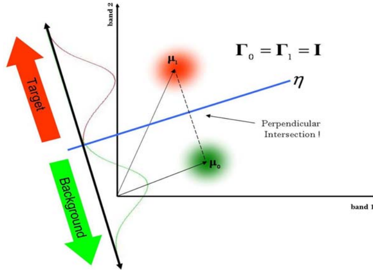
Figure 2.11: Target detector architecture for equal covariances and its transformation into whitened space, illustrating the optimal matched filter target detector concept.
