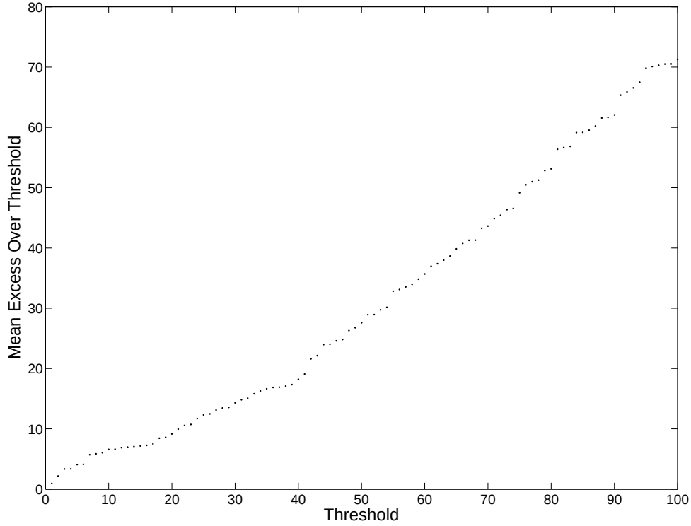
Figure 4.2: A plot of 100 sample mean excess points from 1000 random variables (RVs) generated from a GPD with a positive shape parameter k = 1 , \mu = 0 , and \sigma = 1 . Notice the positive linear slope in the region between u = 40 and u = 90 . The overall positive slope of this plot above the threshold values indicates heavy tail behavior.
