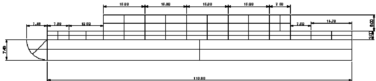
Figure 14. Longitudinal View of Structural Model (the dimensions are in meters)
