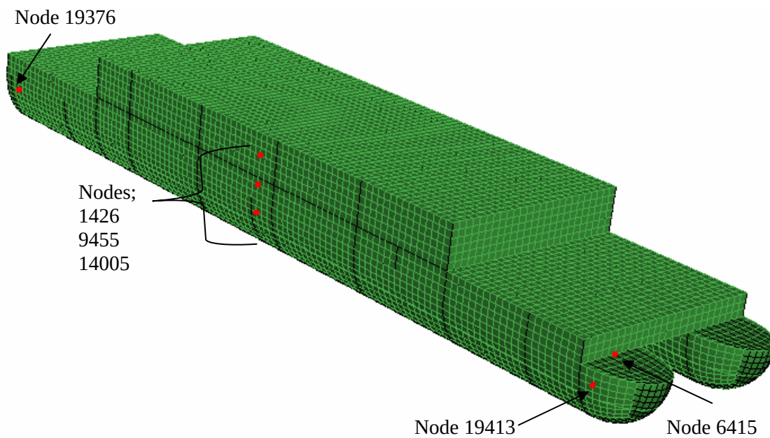
Figure 32. The Location of the Nodes at the Port Side.
