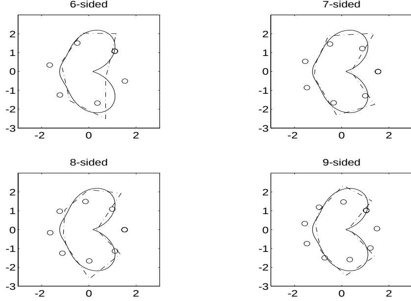
Figure 14: True object (-), reconstruction (-.), initial guess (o) picked using Initial Guess Algorithm, SNR= 4.35 dB.
