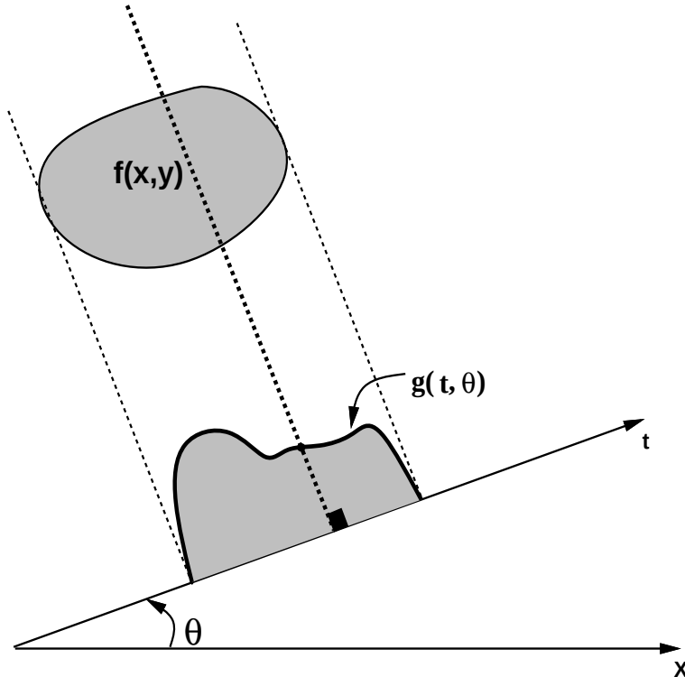
Figure 1: The Radon transform
