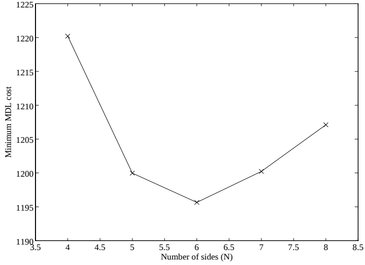
Figure 12: Cost vs number of sides for the hexagon in Figure 5
