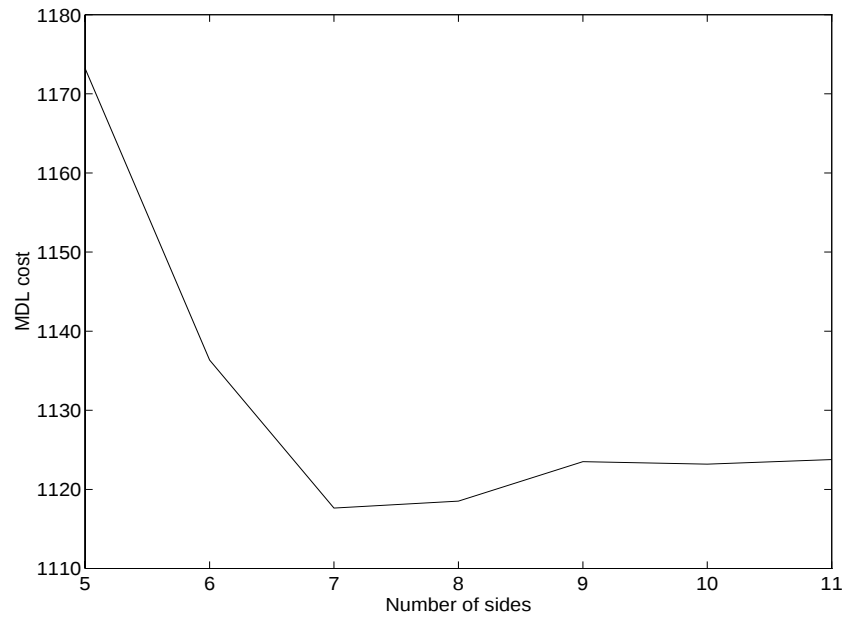
Figure 16: MDL cost curve for the reconstruction of the kidney-shaped object with the Initial Guess Algorithm used.
