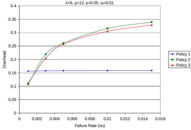
Figure 7.6. Overhead versus failure rate using generalized distributions
