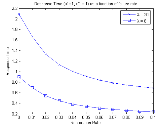
Figure 10.2: Single queue system response time versus failure rate with varied arrival rate
