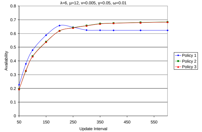
Figure 7.8. Availability versus the update interval
