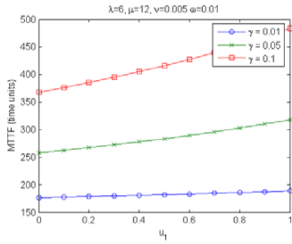
Figure 8.4 Unit MTTF versus control coverage
