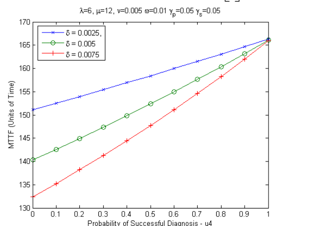
Figure 9. 4 shows the mean time to failure as a function of the conditional probability u_4 with the delay \delta as a parameter. As the probability of successful error diagnosis increases, the mean time to failure also increases. The ability to successfully diagnose errors allows the unit to attend to failures more rapidly. This reduces the ability for another server to fail which results in unit to failure. Also, as the rate of delay increases, the mean time to failure decreases. A smaller delay makes the system easier to enter an intermittent error state. This is particular to the system setup. The
