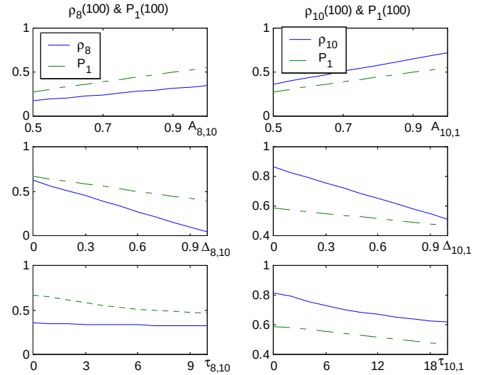
Figure 1.5 Specific reconfigurabilities \rho_8 (left) and \rho_{10} (right) v.s. transition coverage parameters ( A_{8,10} , \Delta_{8,10} , \tau_{8,10} ) and ( A_{10,1} , \Delta_{10,1} , \tau_{10,1} ), respectively.
