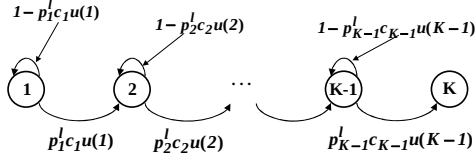
Figure 4.1 Packet transmission in a K -cluster route
