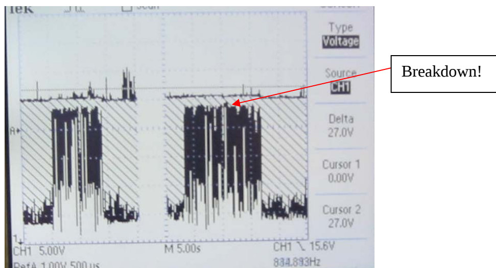
Figure 24. A close-up of the breakdown voltage occurring on the Tektronix TDS 1012
