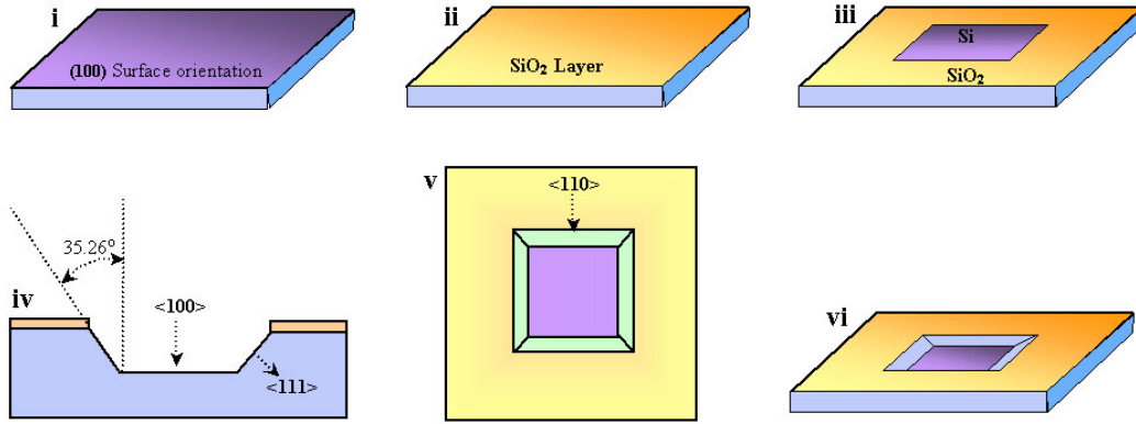
Figure 12. Step diagram showing etching of \text{SiO}_2 wafer 11
