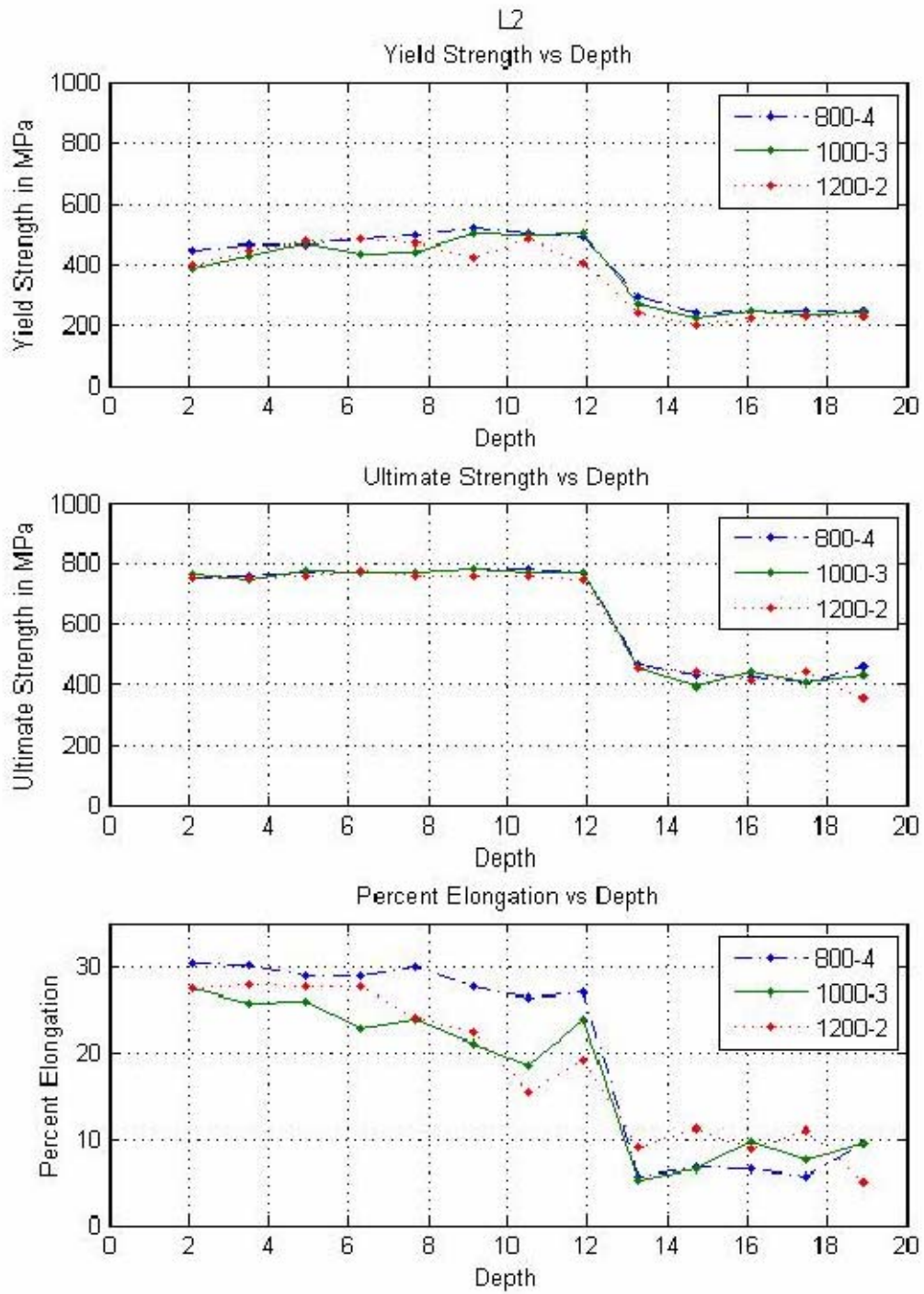
Figure 17. Comparing Material Properties vs. Depth in Tensile Blocks L2; for NAB material FSP with three different RPM/IPM Combinations.
