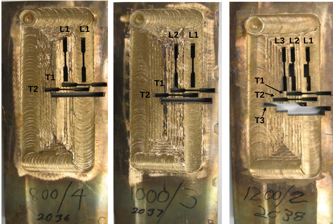
Figure 11. Plates After Cutting Tensile Blocks.
