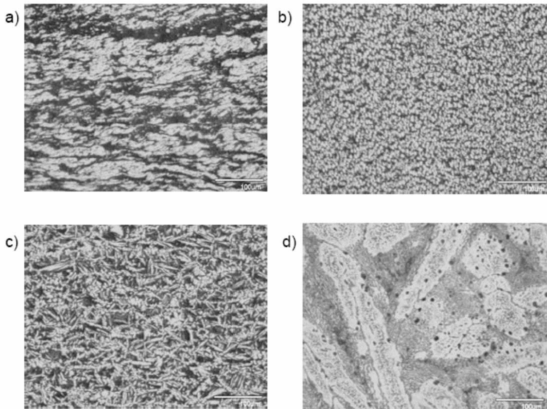
Figure 7. Microstructures created in NAB by FSP, From [10].
