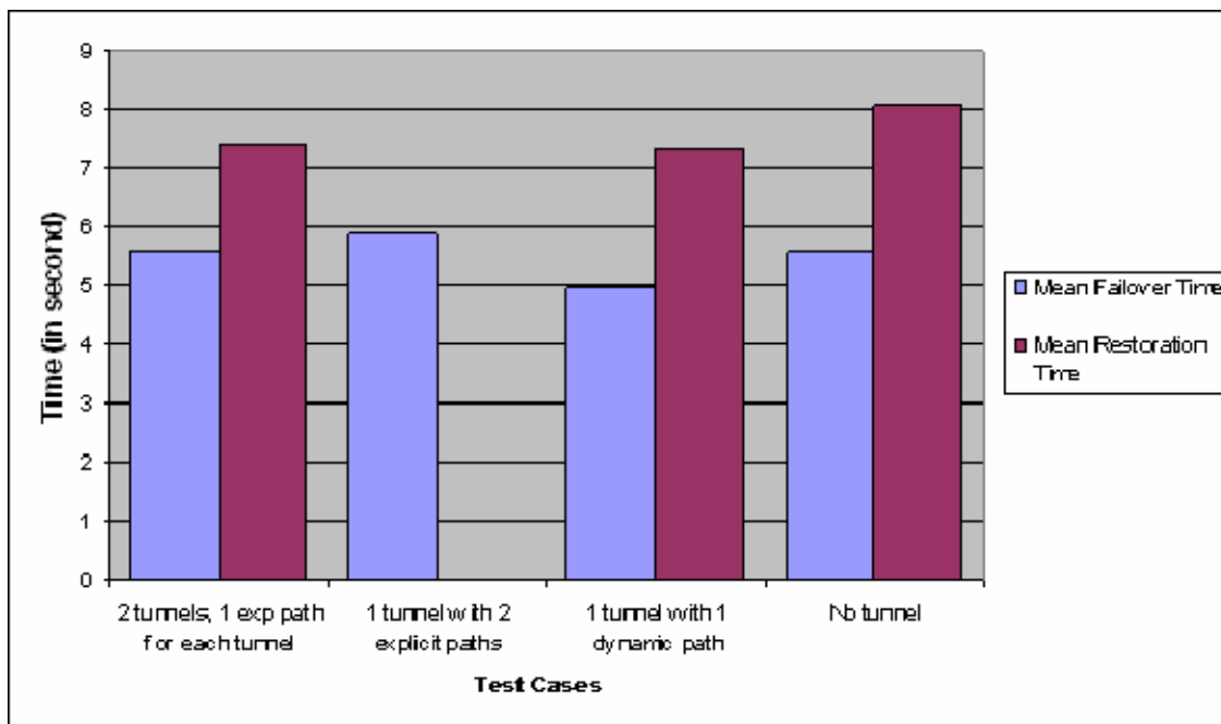
Figure 22. Comparison of Failover and Restoration Time among different TE tunnel configuration options
