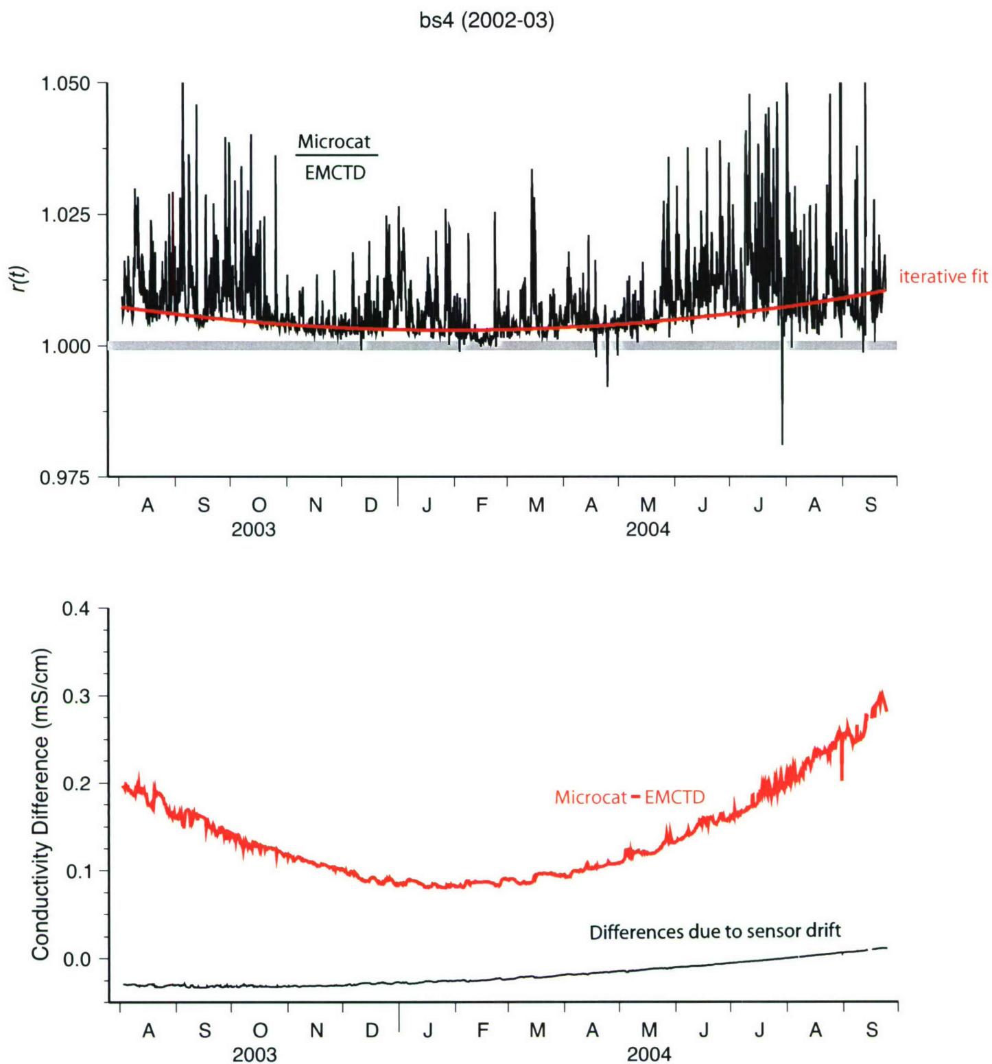
Figure 3: Calibration ratio r(t) and iterative fit for bs4 (2002-03; upper panel). Corresponding conductivity differences between the Microcat and the EMCTD (red; lower panel). The differences due to sensor drift, after the vertical stratification has been accounted for, are shown in black (lower panel).
