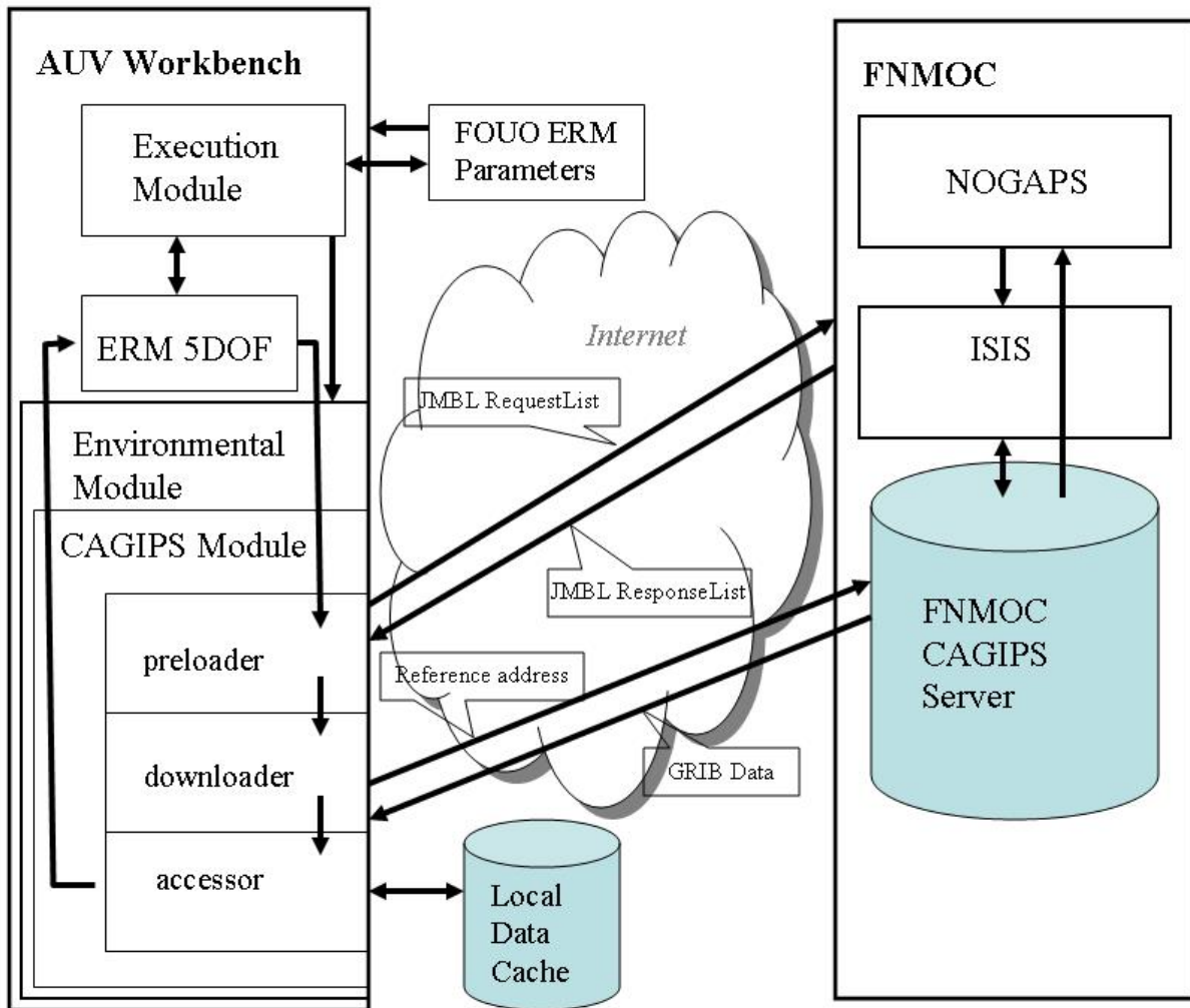
Figure 30. Data flow diagram for BALCOR application.
