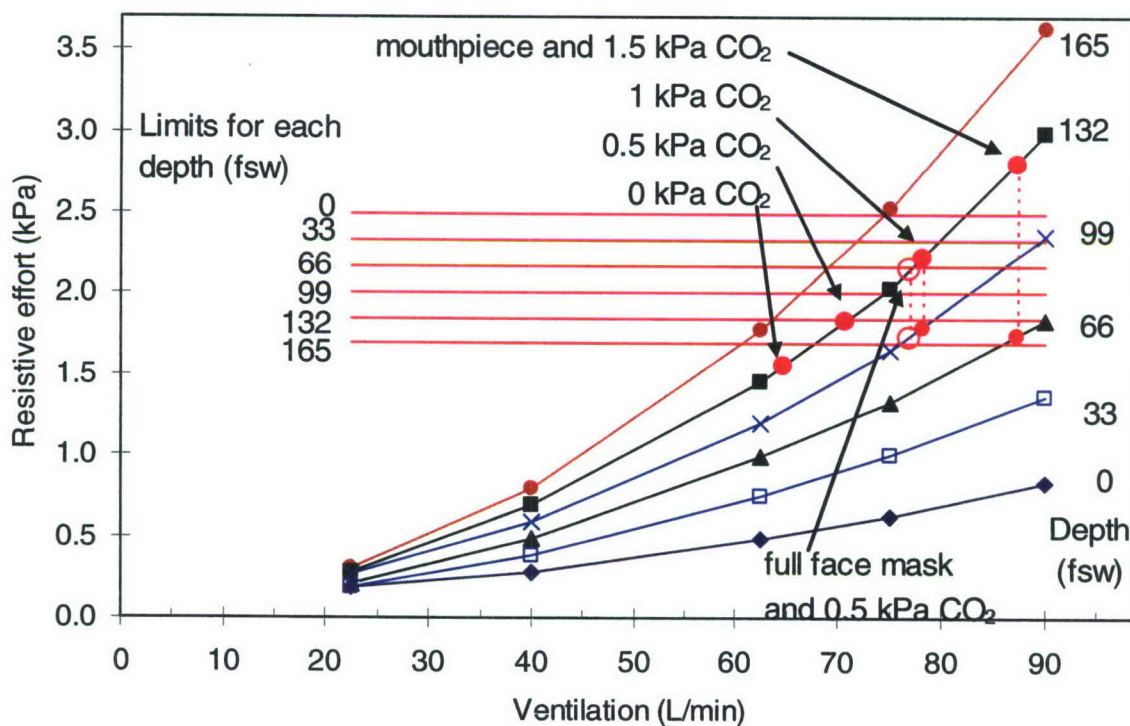
Figure 11. How CO 2 in the inspired gas influences a diver breathing on a UBA with a mouthpiece (red, filled circles) and a full face mask with a well-fitting oronasal cup (red, open circles). Horizontal lines show the proposed limits for resistive effort for each depth. Data are from Figure 5.
