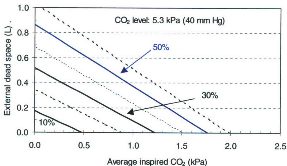
Figure 9. Equivalence between external dead space and average inspired CO 2 for different levels of increased minute ventilation for a diver maintaining a CO 2 level of 5.3 kPa (40 mm Hg).
