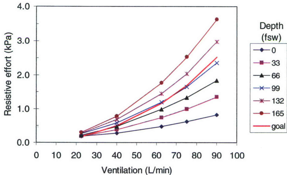
Figure 5. Data plotted together with the current goal for one MK 16 MOD 1 tested in the prone position.
