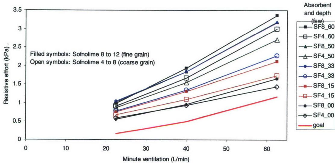
Figure 7. Resistive effort data from one MK 25 UBA plotted against minute ventilation. The current NEDU performance goal is also shown. The MK 25 was tested with two absorbents at depths down to 60 fsw (about 18 msw). In the legend, “SF8” refers to Sofnolime 812® and “SF4” refers to Sofnolime 408®; the numbers “00” through “60” refer to the depth.
