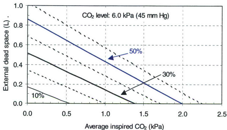
Figure 10. Equivalence between external dead space and average inspired CO 2 for different levels of increased minute ventilation for a diver maintaining a CO 2 level of 6.0 kPa (45 mm Hg).
