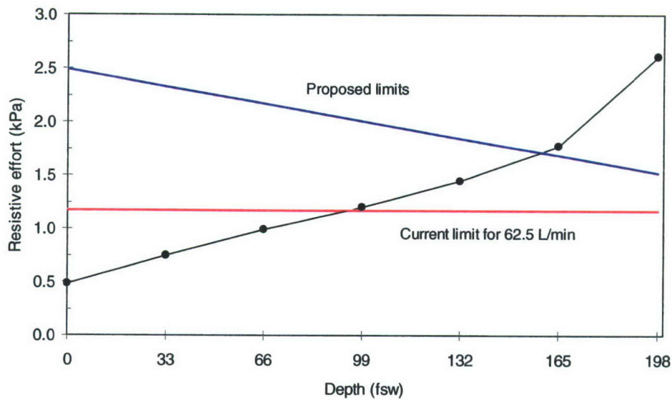
Figure 6. Current performance goal and the proposed limit are plotted together with actual data from one MK 16 MOD 1 tested in the prone position with a minute ventilation of 62.5 L/min.
