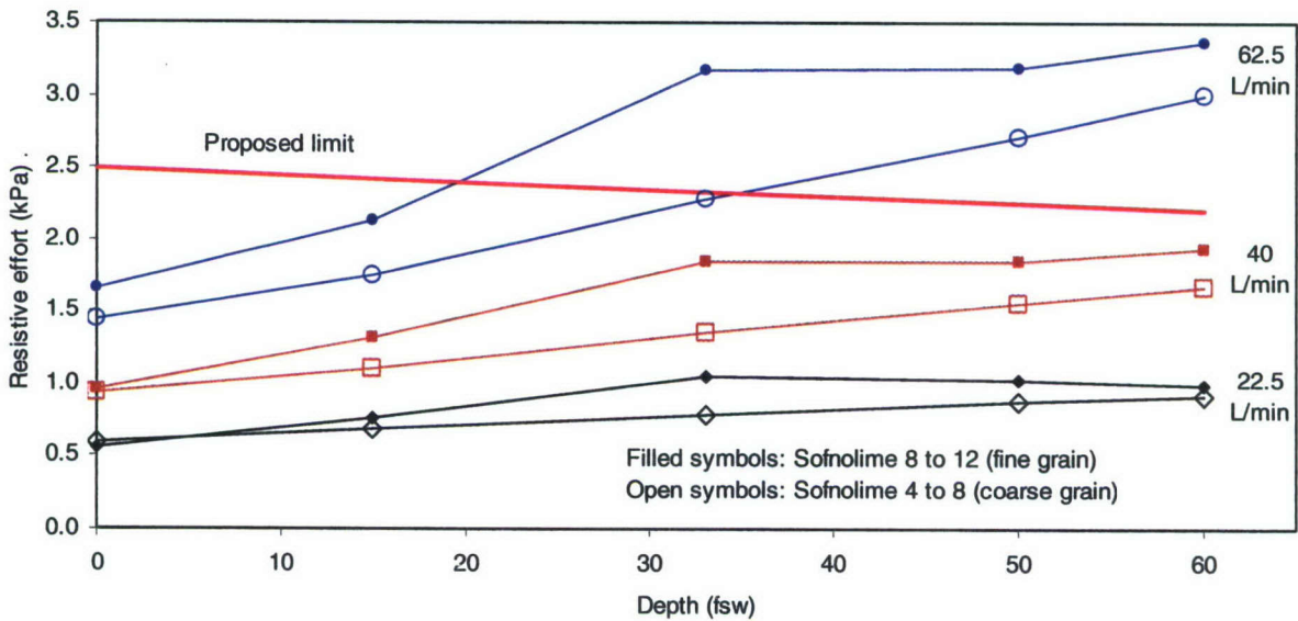
Figure 8. Resistive effort of one MK 25 UBA and the proposed limit plotted against depth. Two absorbents were tested at depths down to 60 fsw (about 18 msw). The statistical analysis has been omitted for clarity.
