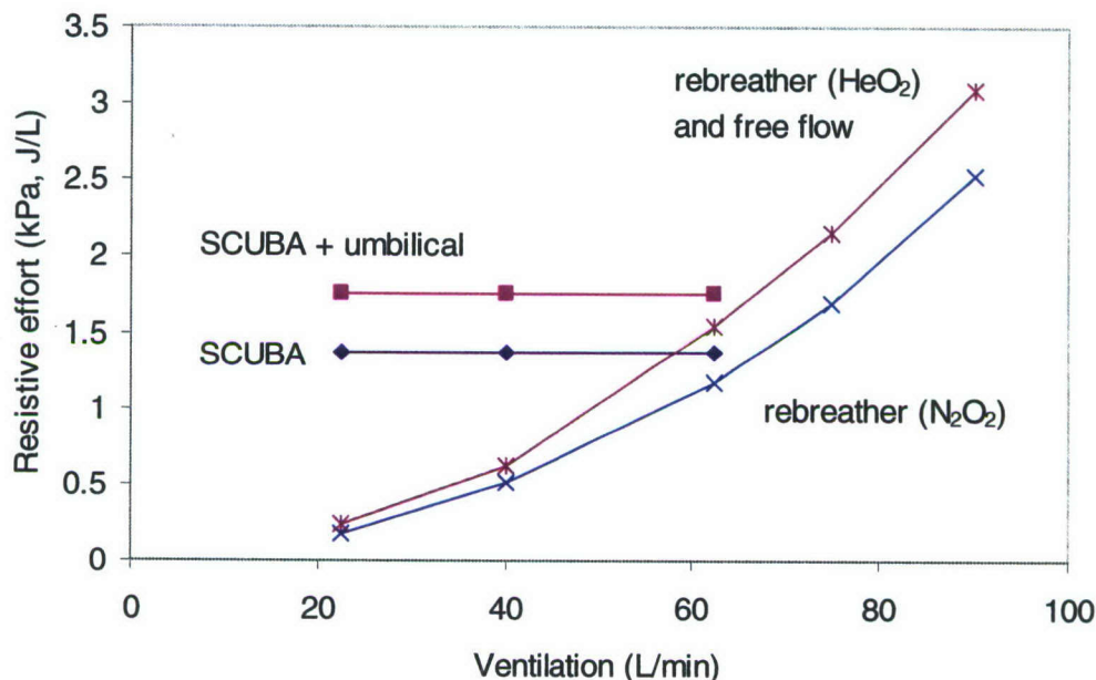
Figure 2. Limits on breathing resistance as proposed by Middleton and Thalmann. 1
