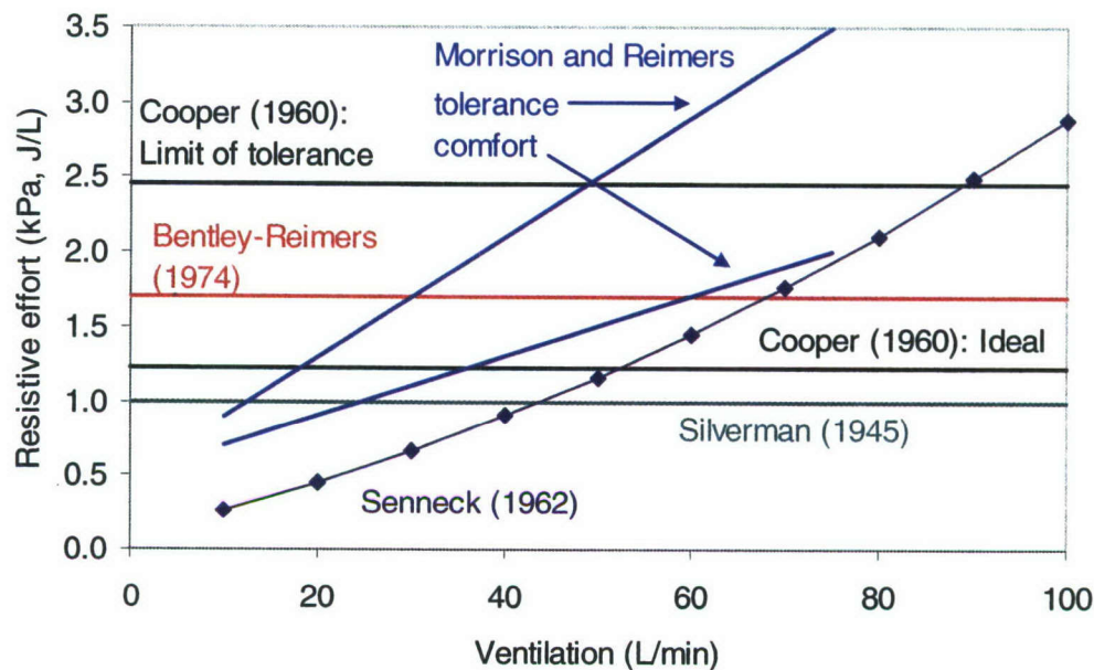
Figure 3. Limits on breathing resistance 6-10 in the review by Morrison and Reimers, 3 with their proposed limits.
