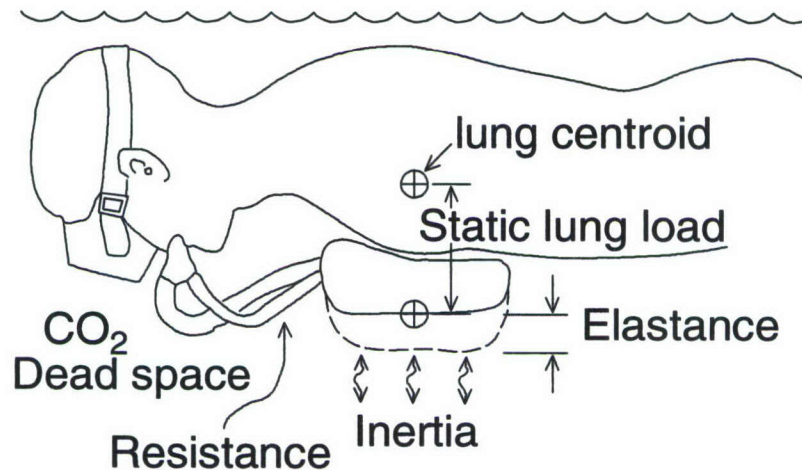
Figure 1. Respiratory loads imposed on a diver breathing a closed-circuit UBA with the breathing bag (counter volume) on the chest.
