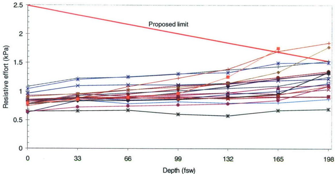
Figure 4. The proposed limit and resistive efforts from 20 regulators breathed at 62.5 L/min. The statistical analysis has been omitted for clarity.
