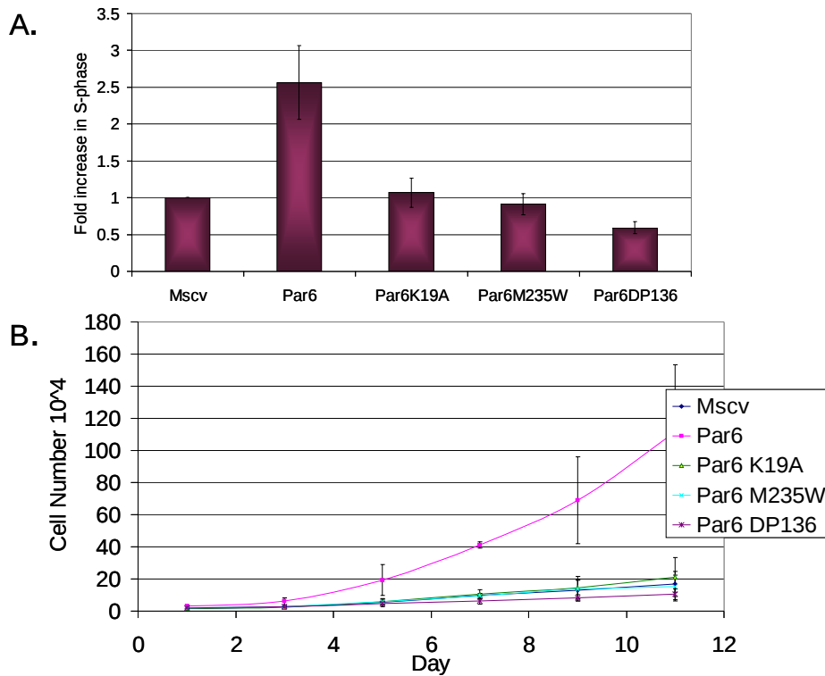
Figure 15. Par6 induced EGF independent proliferation requires aPKC and its effectors. A) S-phase assay was performed as described in Figure 2 with control, Par6, Par6 K19A , Par6 M235W and Par6 Δpro136 . These par6 mutations do not promote EGF independent proliferation. B) Control and mutant Par6 cells were plate and grown over a period of 11 days in EGF free media. Cells were harvested every other day, counted and cell numbers were plotted.
