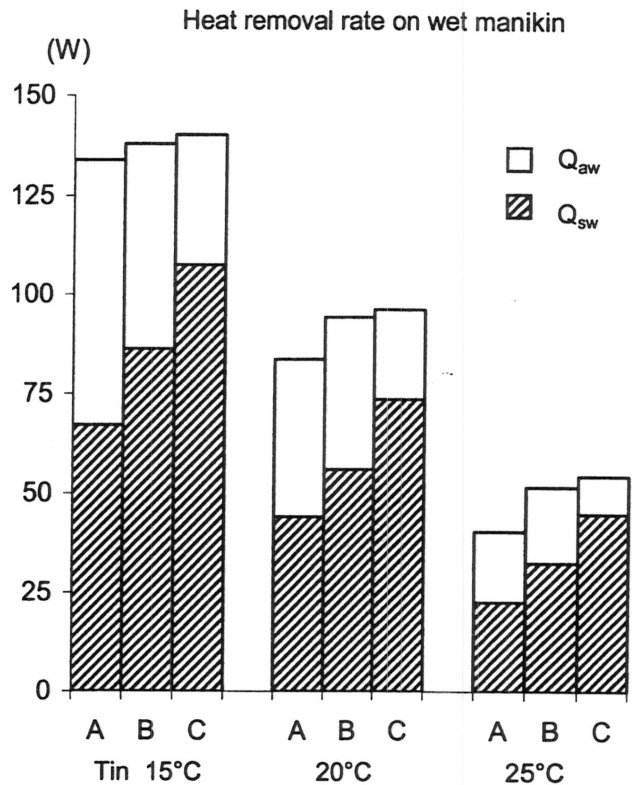
Fig. 3. Heat removal rates for A) the cooling vest (CV); B) CV plus battle dress uniform (CVB); and C) CVB plus battle dress overgarment (CVO) at three water inlet temperatures in the wet (sweating) experiments. Q_{sw} : LCG heat removal from the human body or manikin; Q_{aw} : LCG heat gain from the ambient environment to the LCG.
