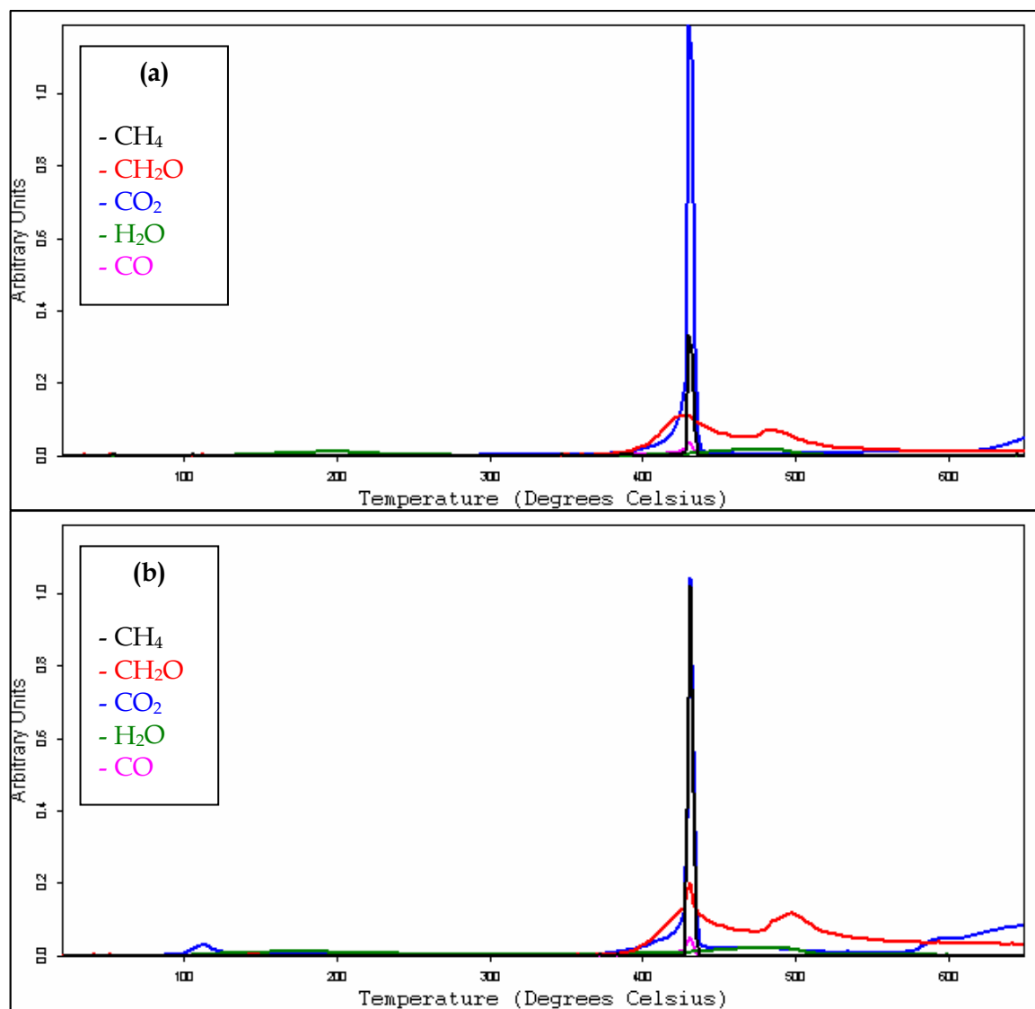
Figure 6 – EGA-FTIR evolved gas profile of 2:1 molar ratio of (a) \text{Fe}_2\text{O}_3 :MPA (b) spent catalyst (used once previously):MPA in oxygen
