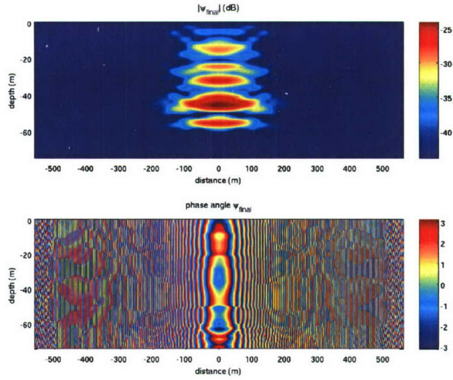
Figure 1. The acoustic field after 500-m propagation through the 60-m deep three-layer environment with no internal waves is shown. Intensity in the tangential cross-range plane is shown at the top, phase in the same plane at the bottom. The beam source has expanded to fill a lateral distance of 200 m, indicating a beam width of about 22 degrees.
